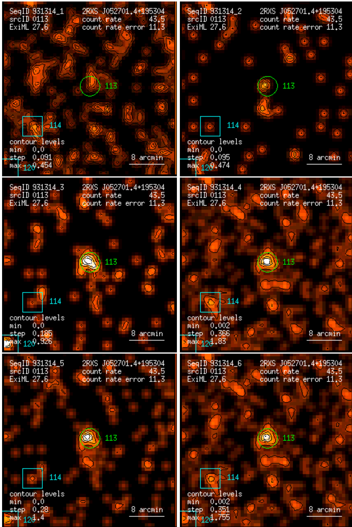
Figure 113: RASS 931314: detection 0113: band rate images, Gaussian filter: (1) PSPC channels 11 – 41, (2) 52 – 90, (3) 91 – 201, (4) 11 – 235, (5) 52 – 201, (6) 11 – 201. Broad band rates in counts/ks. Band rate contour levels in counts/ks/arcmin 2 .
