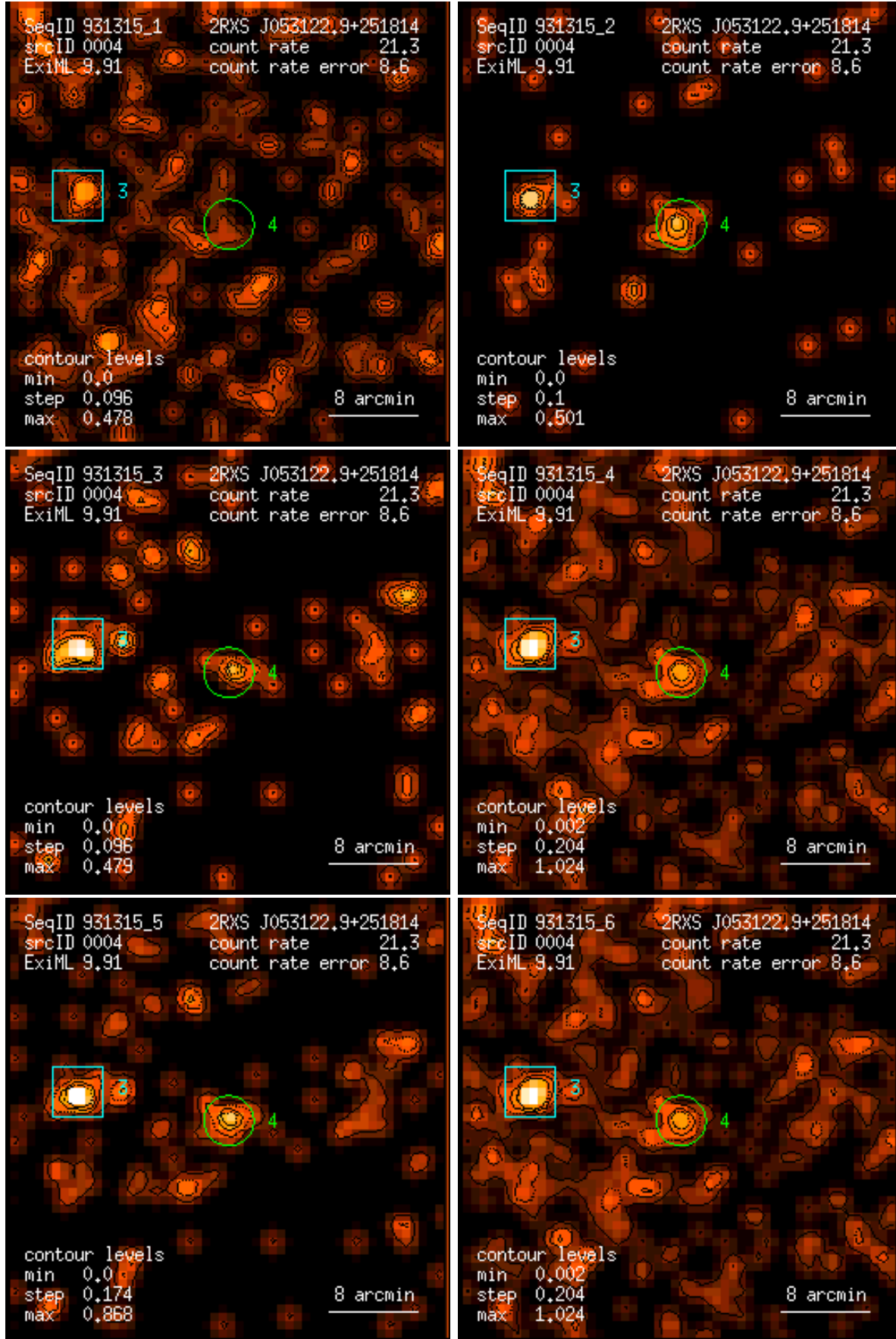
Figure 4: RASS 931315: detection 0004: band rate images, Gaussian filter: (1) PSPC channels 11 – 41, (2) 52 – 90, (3) 91 – 201, (4) 11 – 235, (5) 52 – 201, (6) 11 – 201. Broad band rates in counts/ks. Band rate contour levels in counts/ks/arcmin 2 .
