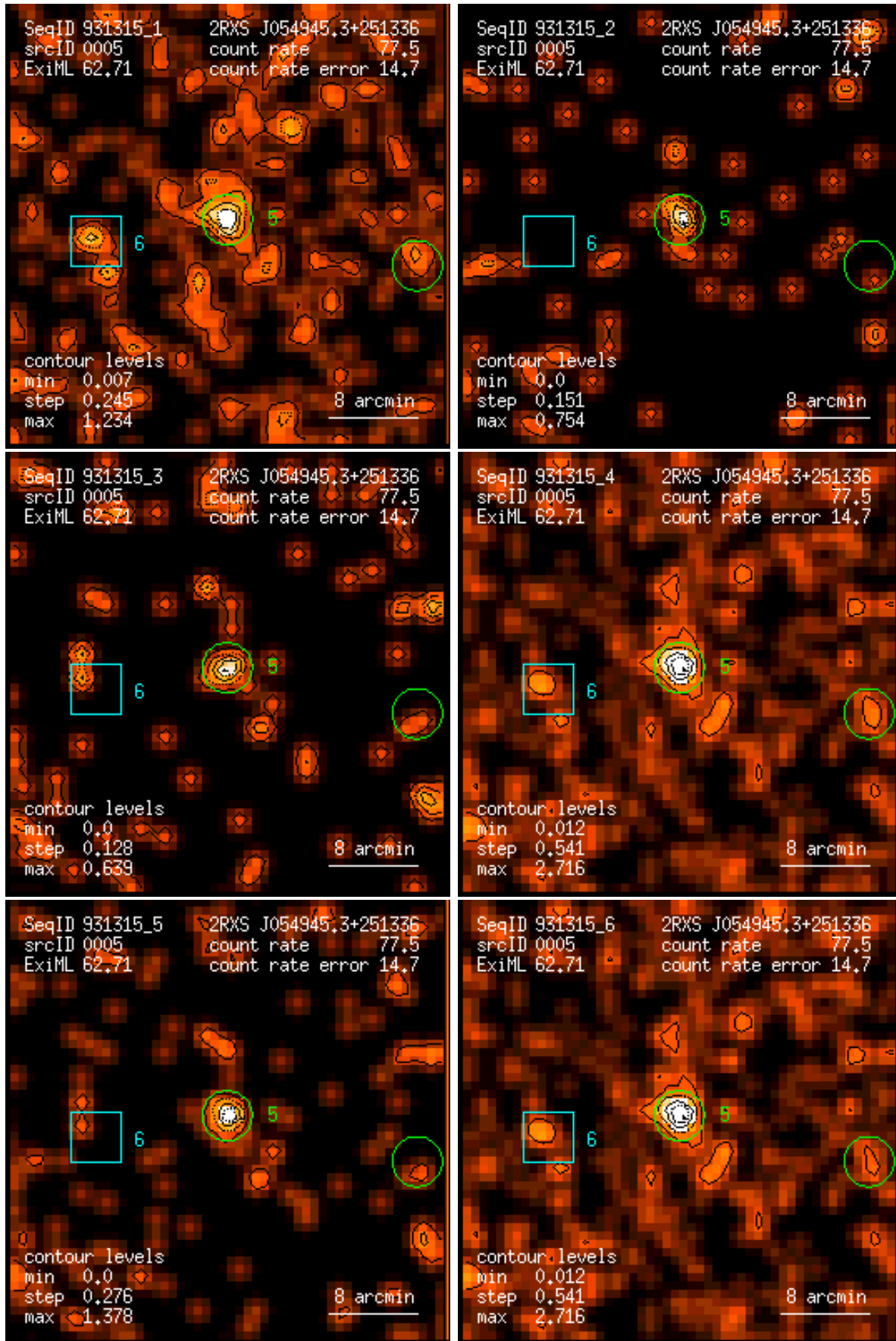
Figure 5: RASS 931315: detection 0005: band rate images, Gaussian filter: (1) PSPC channels 11 – 41, (2) 52 – 90, (3) 91 – 201, (4) 11 – 235, (5) 52 – 201, (6) 11 – 201. Broad band rates in counts/ks. Band rate contour levels in counts/ks/arcmin 2 .
