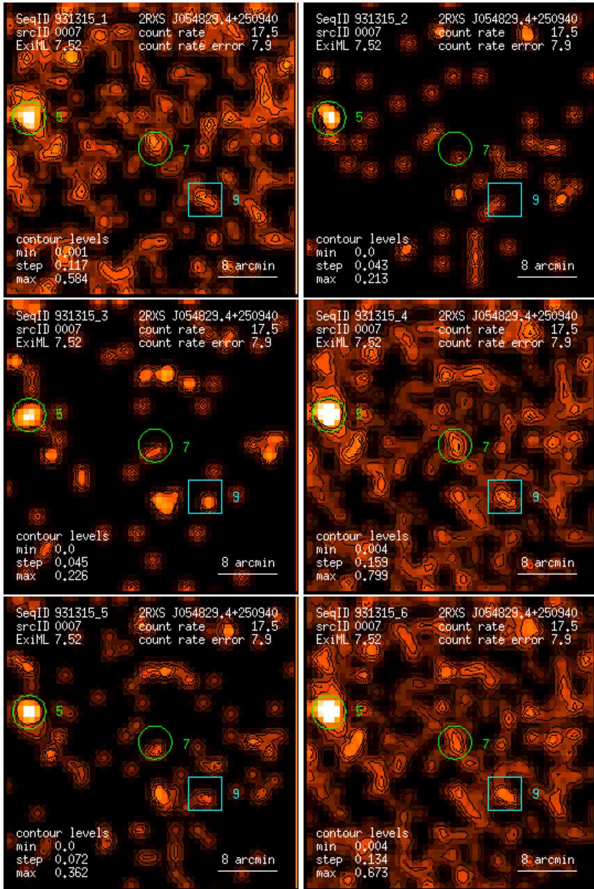
Figure 7: RASS 931315: detection 0007: band rate images, Gaussian filter: (1) PSPC channels 11 – 41, (2) 52 – 90, (3) 91 – 201, (4) 11 – 235, (5) 52 – 201, (6) 11 – 201. Broad band rates in counts/ks. Band rate contour levels in counts/ks/arcmin 2 .
