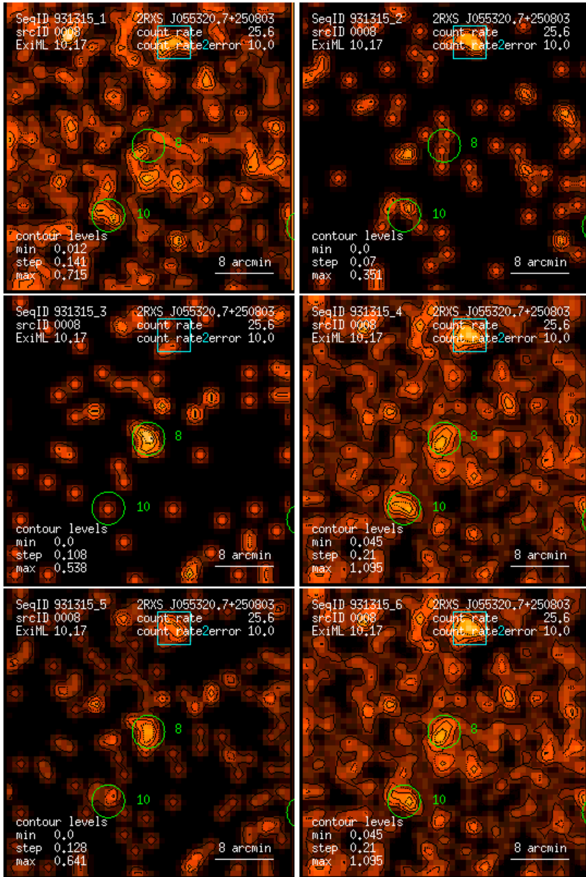
Figure 8: RASS 931315: detection 0008: band rate images, Gaussian filter: (1) PSPC channels 11 – 41, (2) 52 – 90, (3) 91 – 201, (4) 11 – 235, (5) 52 – 201, (6) 11 – 201. Broad band rates in counts/ks. Band rate contour levels in counts/ks/arcmin 2 .
