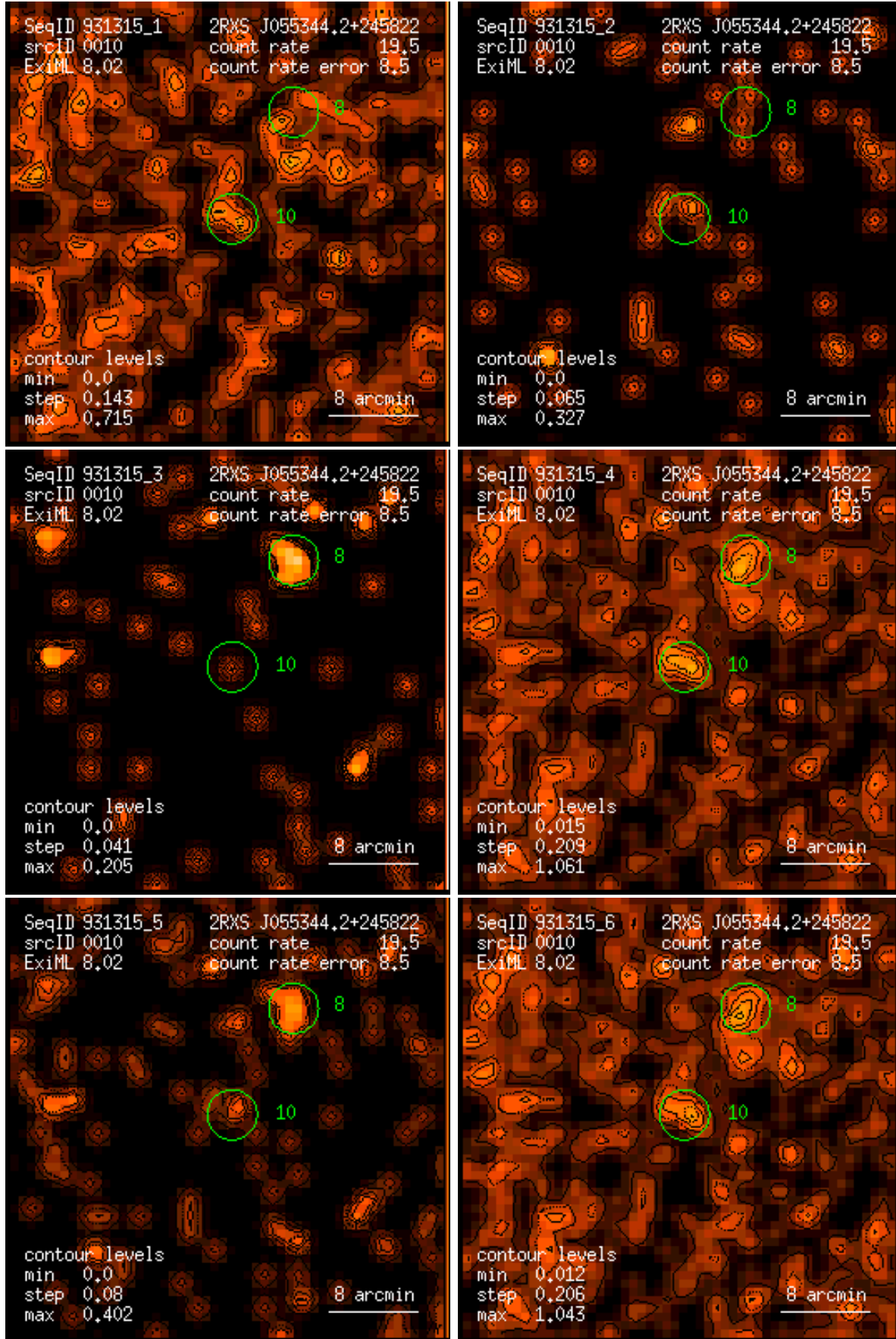
Figure 10: RASS 931315: detection 0010: band rate images, Gaussian filter: (1) PSPC channels 11 – 41, (2) 52 – 90, (3) 91 – 201, (4) 11 – 235, (5) 52 – 201, (6) 11 – 201. Broad band rates in counts/ks. Band rate contour levels in counts/ks/arcmin 2 .
