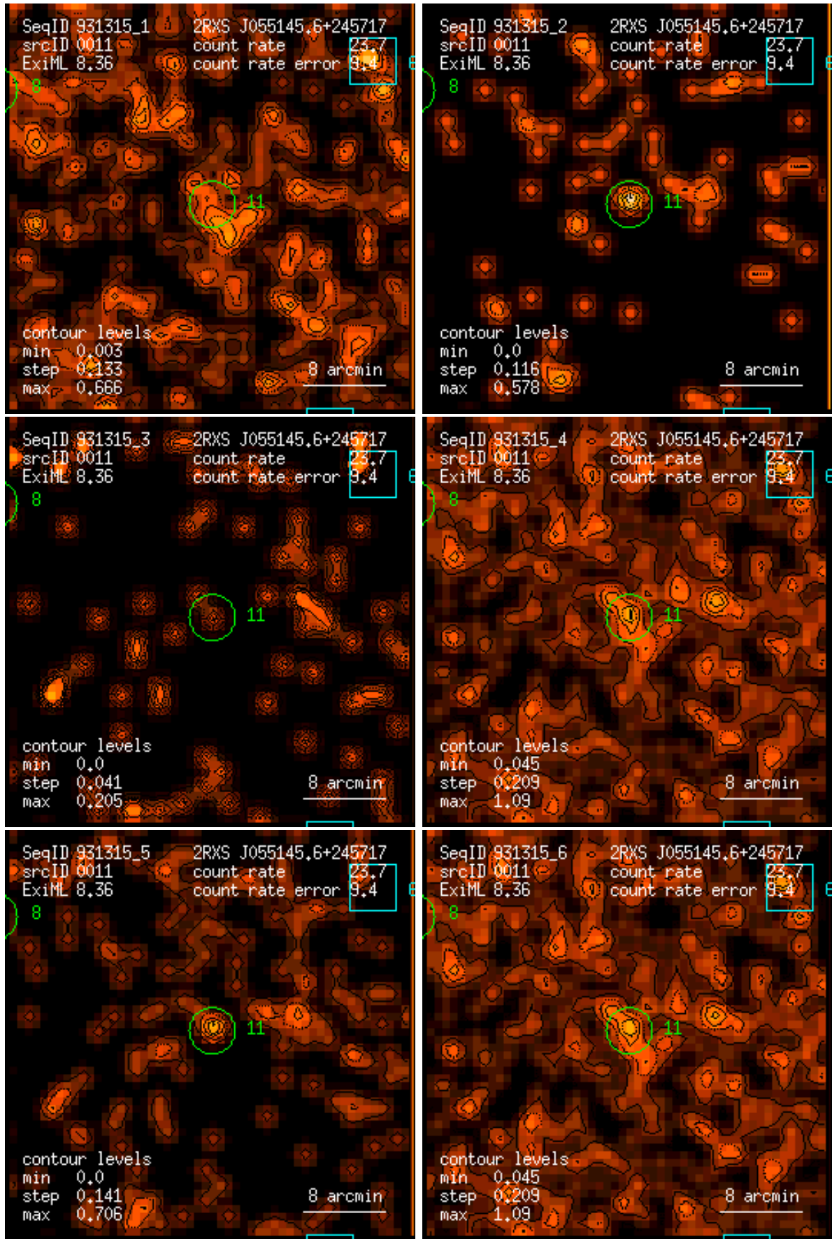
Figure 11: RASS 931315: detection 0011: band rate images, Gaussian filter: (1) PSPC channels 11 – 41, (2) 52 – 90, (3) 91 – 201, (4) 11 – 235, (5) 52 – 201, (6) 11 – 201. Broad band rates in counts/ks. Band rate contour levels in counts/ks/arcmin 2 .
