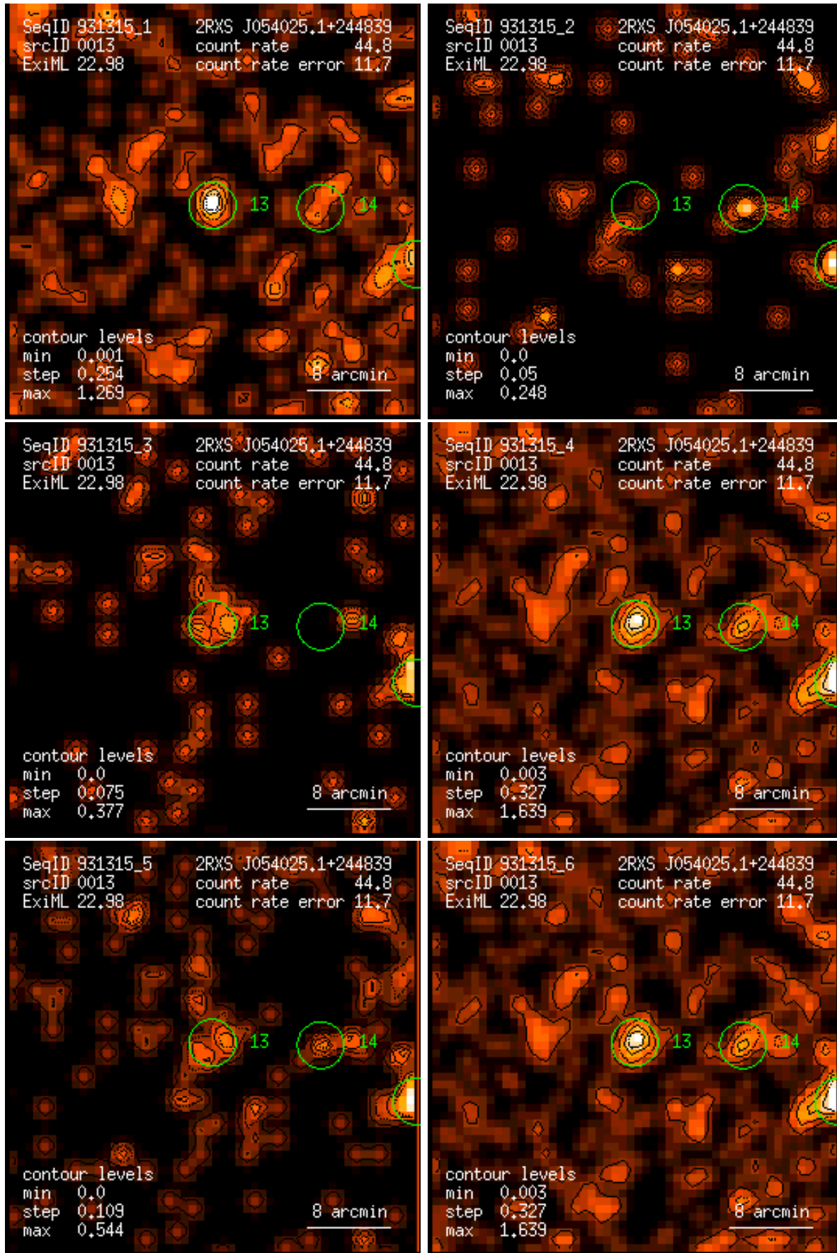
Figure 13: RASS 931315: detection 0013: band rate images, Gaussian filter: (1) PSPC channels 11 – 41, (2) 52 – 90, (3) 91 – 201, (4) 11 – 235, (5) 52 – 201, (6) 11 – 201. Broad band rates in counts/ks. Band rate contour levels in counts/ks/arcmin 2 .
