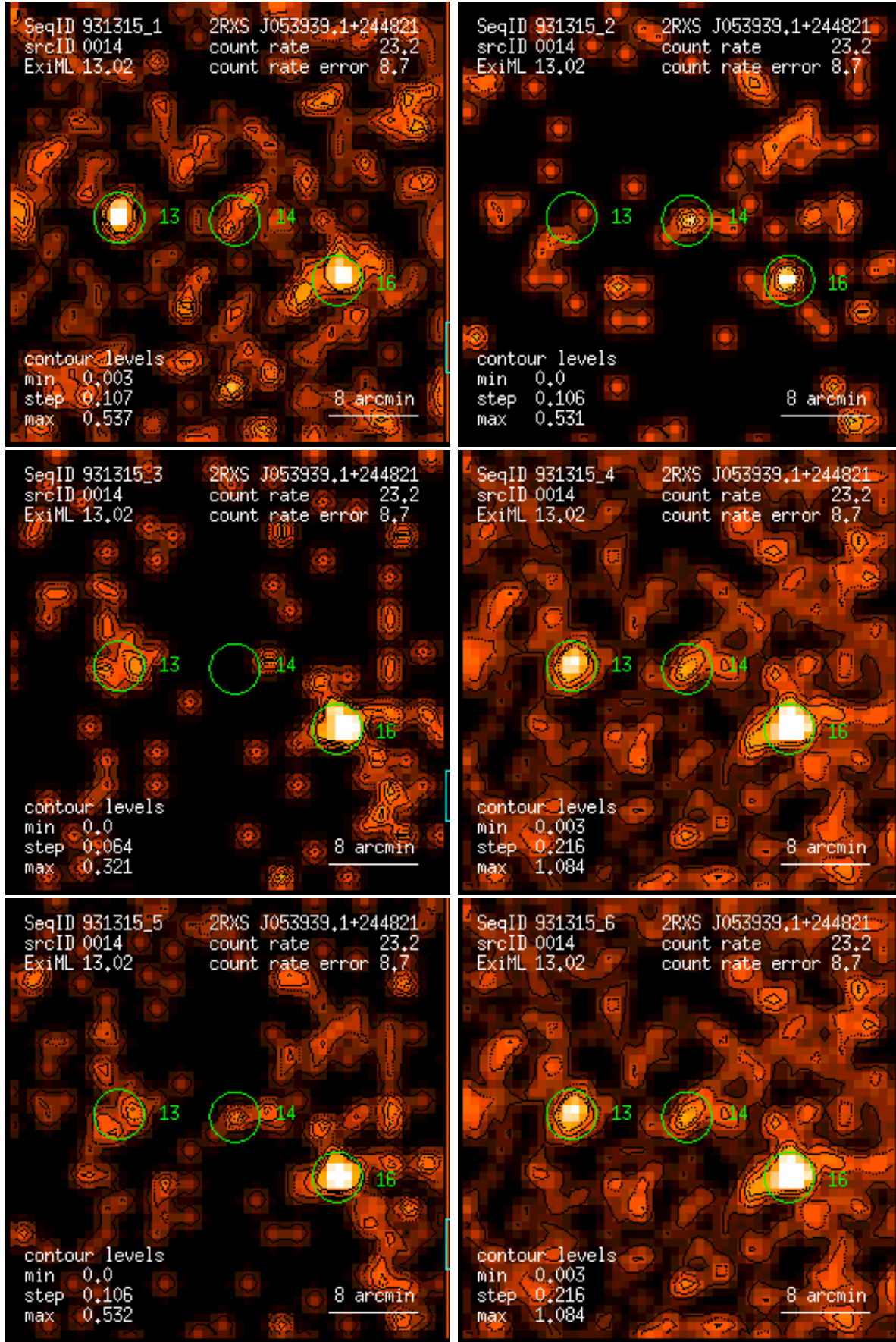
Figure 14: RASS 931315: detection 0014: band rate images, Gaussian filter: (1) PSPC channels 11 – 41, (2) 52 – 90, (3) 91 – 201, (4) 11 – 235, (5) 52 – 201, (6) 11 – 201. Broad band rates in counts/ks. Band rate contour levels in counts/ks/arcmin 2 .
