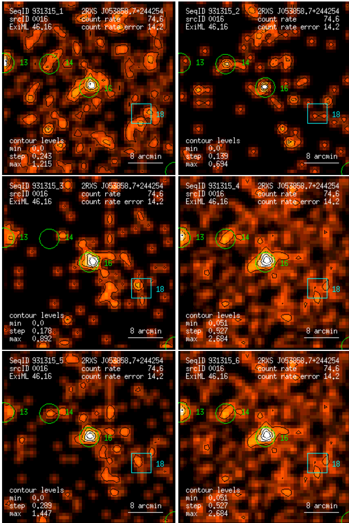
Figure 16: RASS 931315: detection 0016: band rate images, Gaussian filter: (1) PSPC channels 11 – 41, (2) 52 – 90, (3) 91 – 201, (4) 11 – 235, (5) 52 – 201, (6) 11 – 201. Broad band rates in counts/ks. Band rate contour levels in counts/ks/arcmin 2 .
