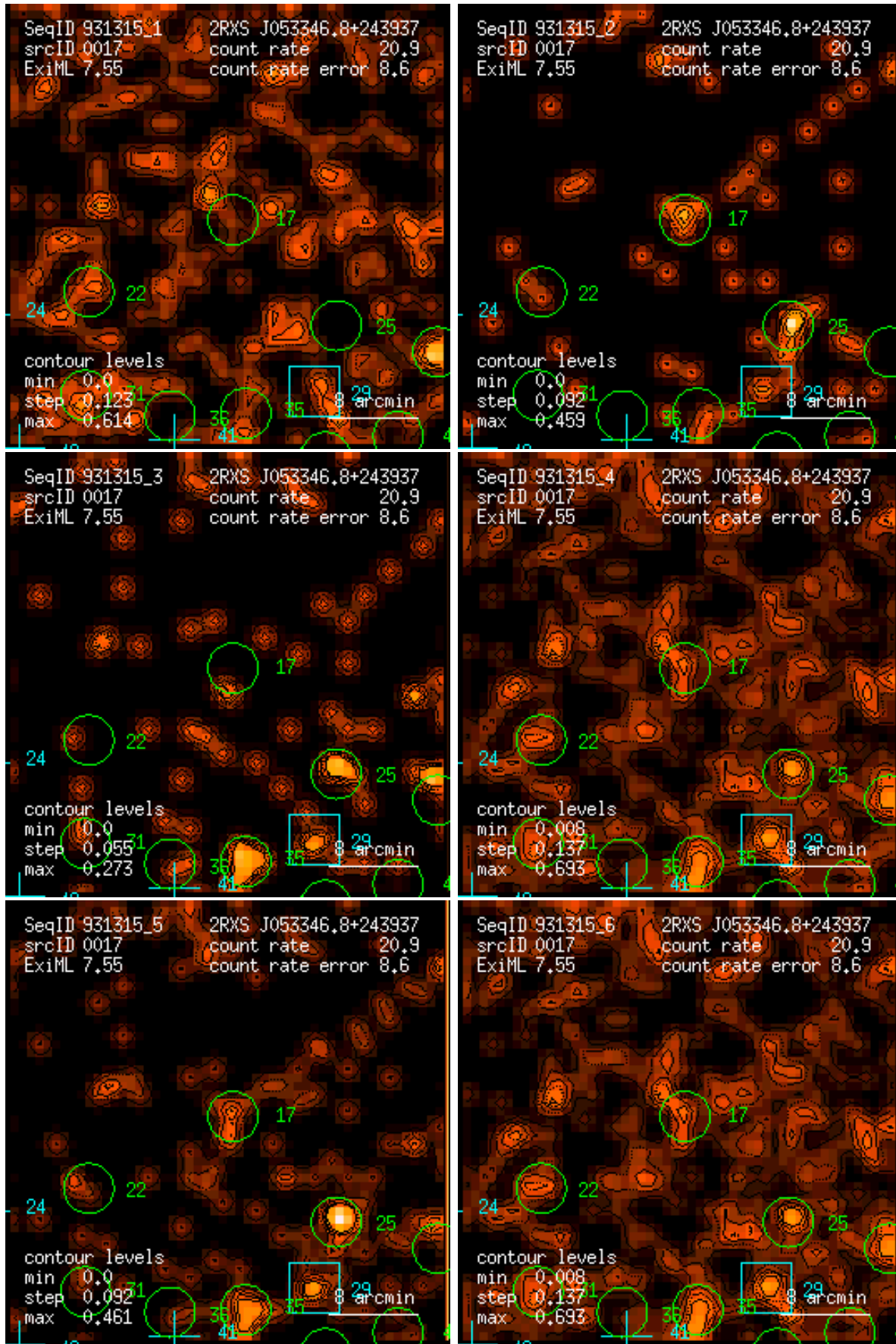
Figure 17: RASS 931315: detection 0017: band rate images, Gaussian filter: (1) PSPC channels 11 – 41, (2) 52 – 90, (3) 91 – 201, (4) 11 – 235, (5) 52 – 201, (6) 11 – 201. Broad band rates in counts/ks. Band rate contour levels in counts/ks/arcmin 2 .
