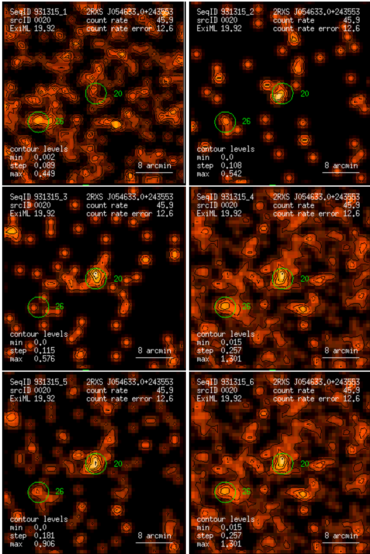
Figure 20: RASS 931315: detection 0020: band rate images, Gaussian filter: (1) PSPC channels 11 – 41, (2) 52 – 90, (3) 91 – 201, (4) 11 – 235, (5) 52 – 201, (6) 11 – 201. Broad band rates in counts/ks. Band rate contour levels in counts/ks/arcmin 2 .
