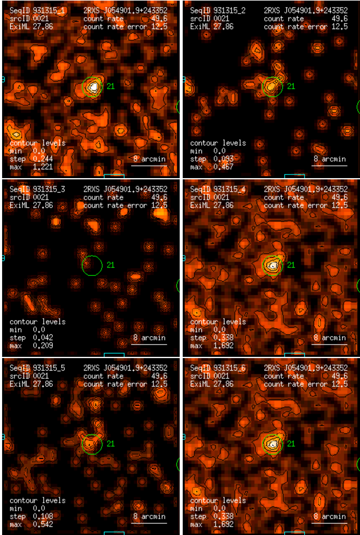
Figure 21: RASS 931315: detection 0021: band rate images, Gaussian filter: (1) PSPC channels 11 – 41, (2) 52 – 90, (3) 91 – 201, (4) 11 – 235, (5) 52 – 201, (6) 11 – 201. Broad band rates in counts/ks. Band rate contour levels in counts/ks/arcmin 2 .
