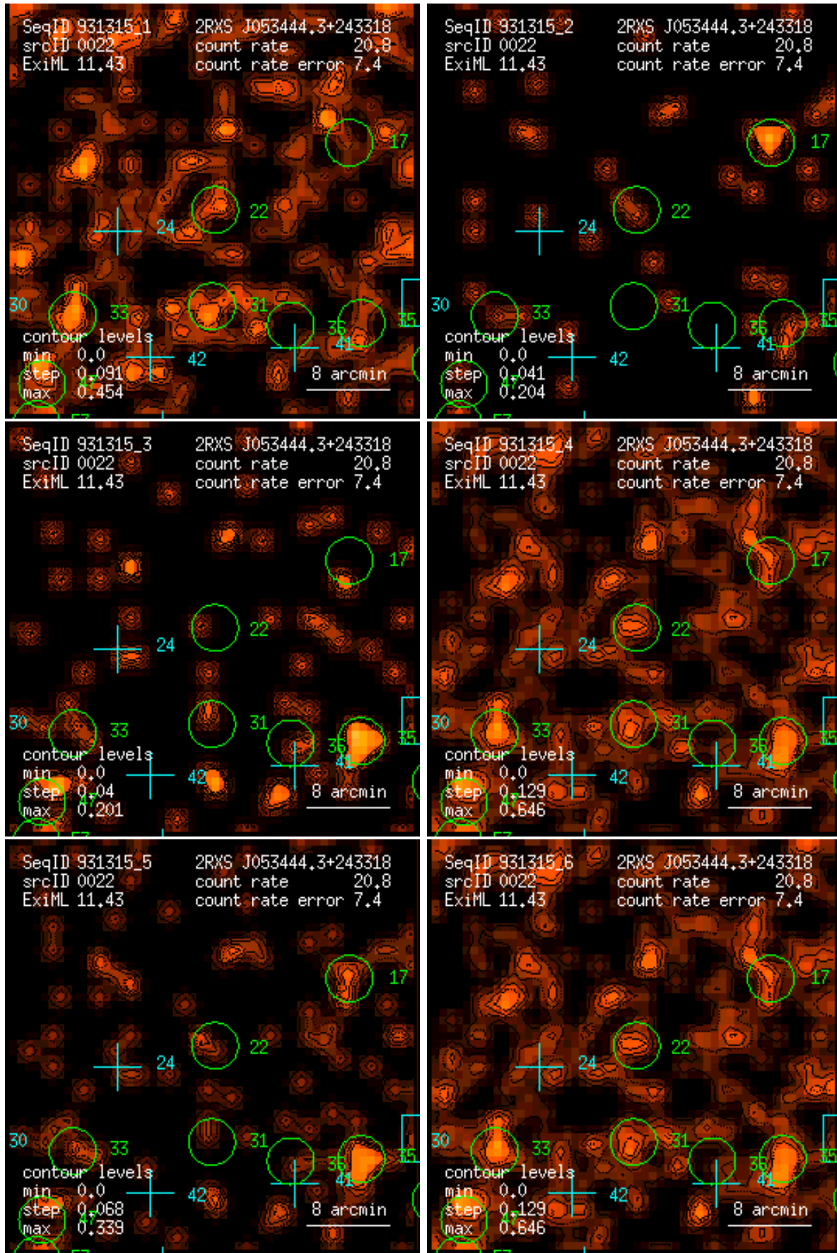
Figure 22: RASS 931315: detection 0022: band rate images, Gaussian filter: (1) PSPC channels 11 – 41, (2) 52 – 90, (3) 91 – 201, (4) 11 – 235, (5) 52 – 201, (6) 11 – 201. Broad band rates in counts/ks. Band rate contour levels in counts/ks/arcmin 2 .
