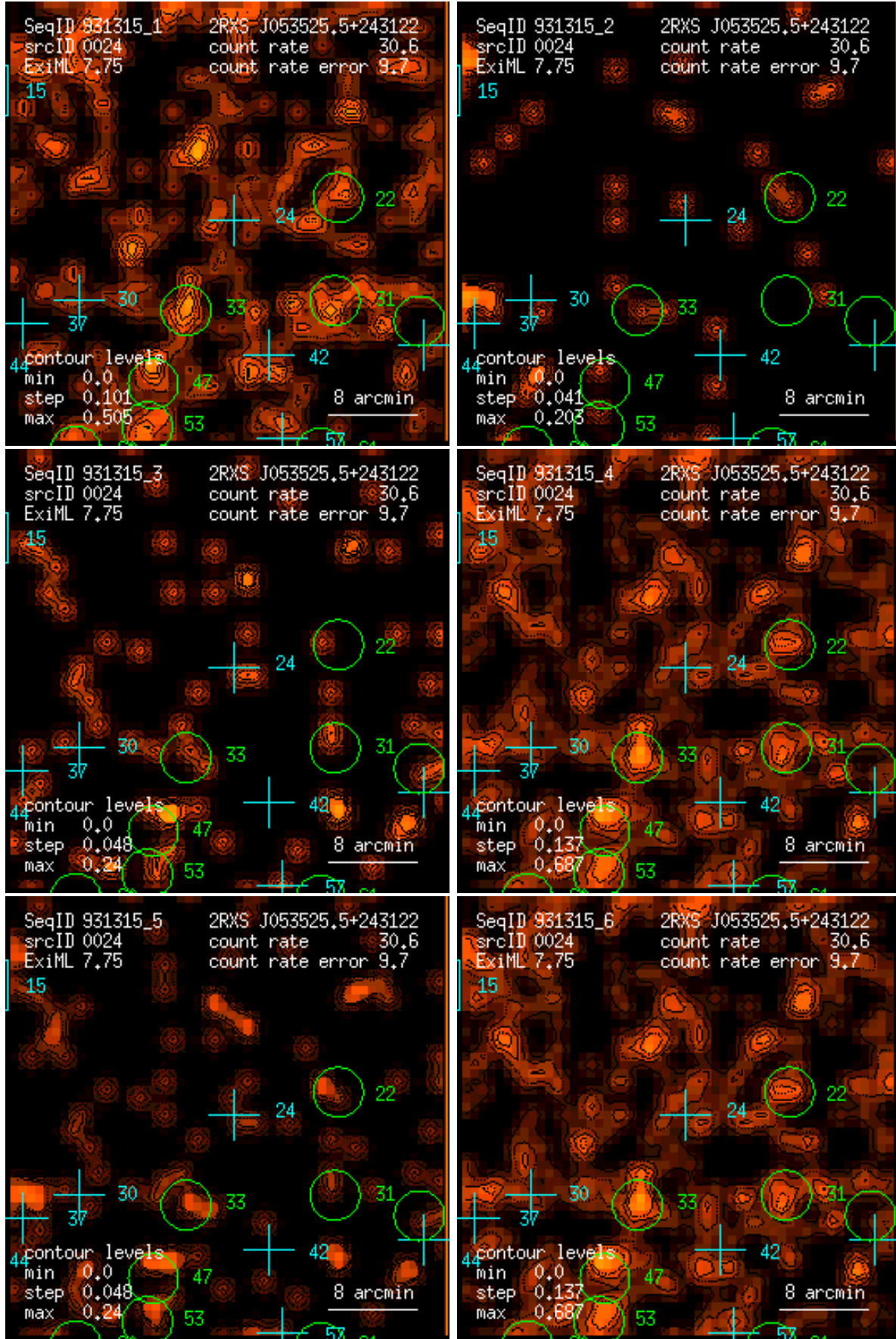
Figure 24: RASS 931315: detection 0024: band rate images, Gaussian filter: (1) PSPC channels 11 – 41, (2) 52 – 90, (3) 91 – 201, (4) 11 – 235, (5) 52 – 201, (6) 11 – 201. Broad band rates in counts/ks. Band rate contour levels in counts/ks/arcmin 2 .
