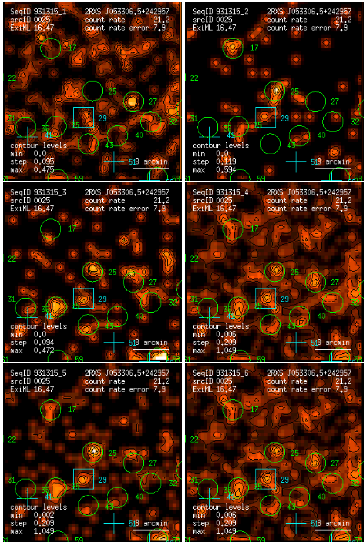
Figure 25: RASS 931315: detection 0025: band rate images, Gaussian filter: (1) PSPC channels 11 – 41, (2) 52 – 90, (3) 91 – 201, (4) 11 – 235, (5) 52 – 201, (6) 11 – 201. Broad band rates in counts/ks. Band rate contour levels in counts/ks/arcmin 2 .
