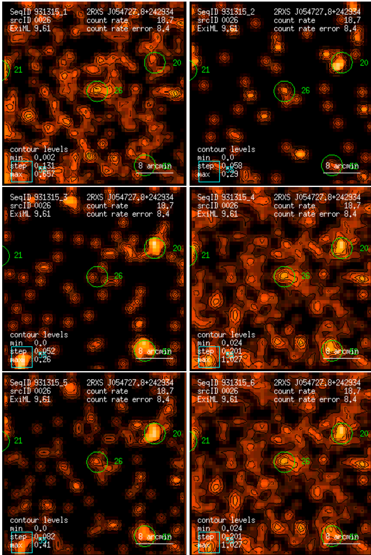
Figure 26: RASS 931315: detection 0026: band rate images, Gaussian filter: (1) PSPC channels 11 – 41, (2) 52 – 90, (3) 91 – 201, (4) 11 – 235, (5) 52 – 201, (6) 11 – 201. Broad band rates in counts/ks. Band rate contour levels in counts/ks/arcmin 2 .
