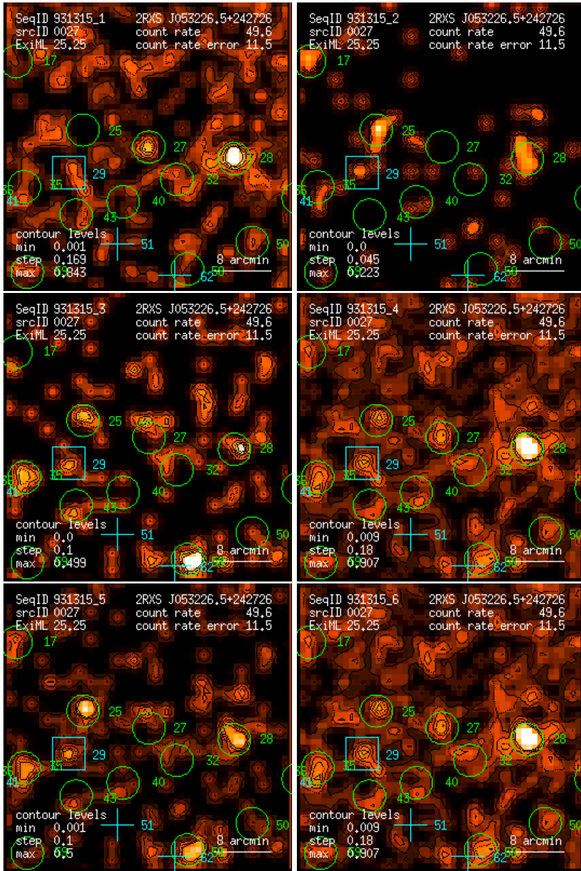
Figure 27: RASS 931315: detection 0027: band rate images, Gaussian filter: (1) PSPC channels 11 – 41, (2) 52 – 90, (3) 91 – 201, (4) 11 – 235, (5) 52 – 201, (6) 11 – 201. Broad band rates in counts/ks. Band rate contour levels in counts/ks/arcmin 2 .
