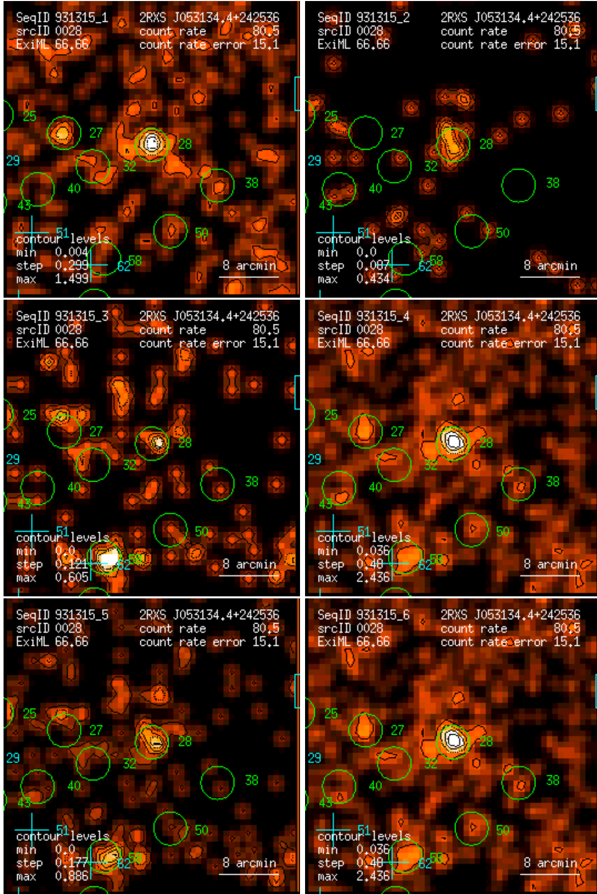
Figure 28: RASS 931315: detection 0028: band rate images, Gaussian filter: (1) PSPC channels 11 – 41, (2) 52 – 90, (3) 91 – 201, (4) 11 – 235, (5) 52 – 201, (6) 11 – 201. Broad band rates in counts/ks. Band rate contour levels in counts/ks/arcmin 2 .
