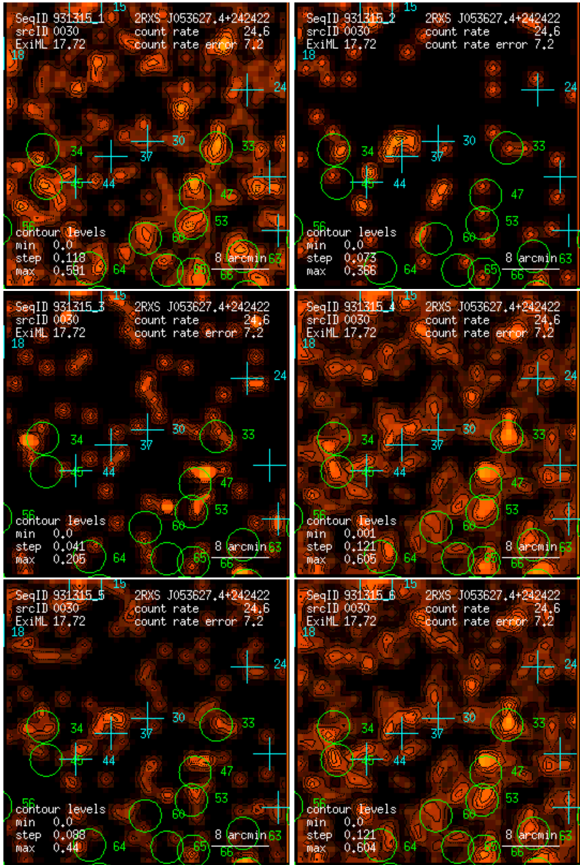
Figure 30: RASS 931315: detection 0030: band rate images, Gaussian filter: (1) PSPC channels 11 – 41, (2) 52 – 90, (3) 91 – 201, (4) 11 – 235, (5) 52 – 201, (6) 11 – 201. Broad band rates in counts/ks. Band rate contour levels in counts/ks/arcmin 2 .
