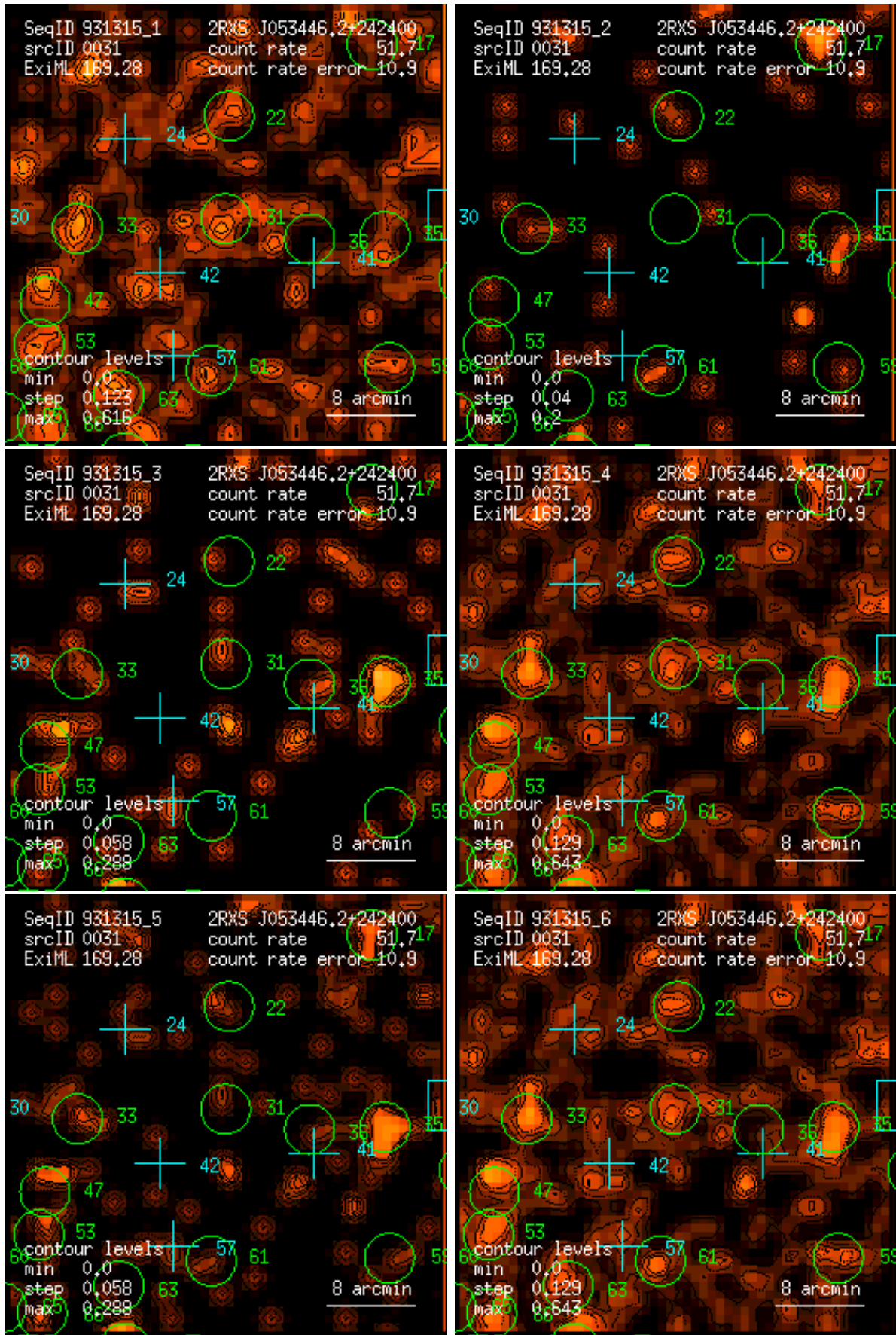
Figure 31: RASS 931315: detection 0031: band rate images, Gaussian filter: (1) PSPC channels 11 – 41, (2) 52 – 90, (3) 91 – 201, (4) 11 – 235, (5) 52 – 201, (6) 11 – 201. Broad band rates in counts/ks. Band rate contour levels in counts/ks/arcmin 2 .
