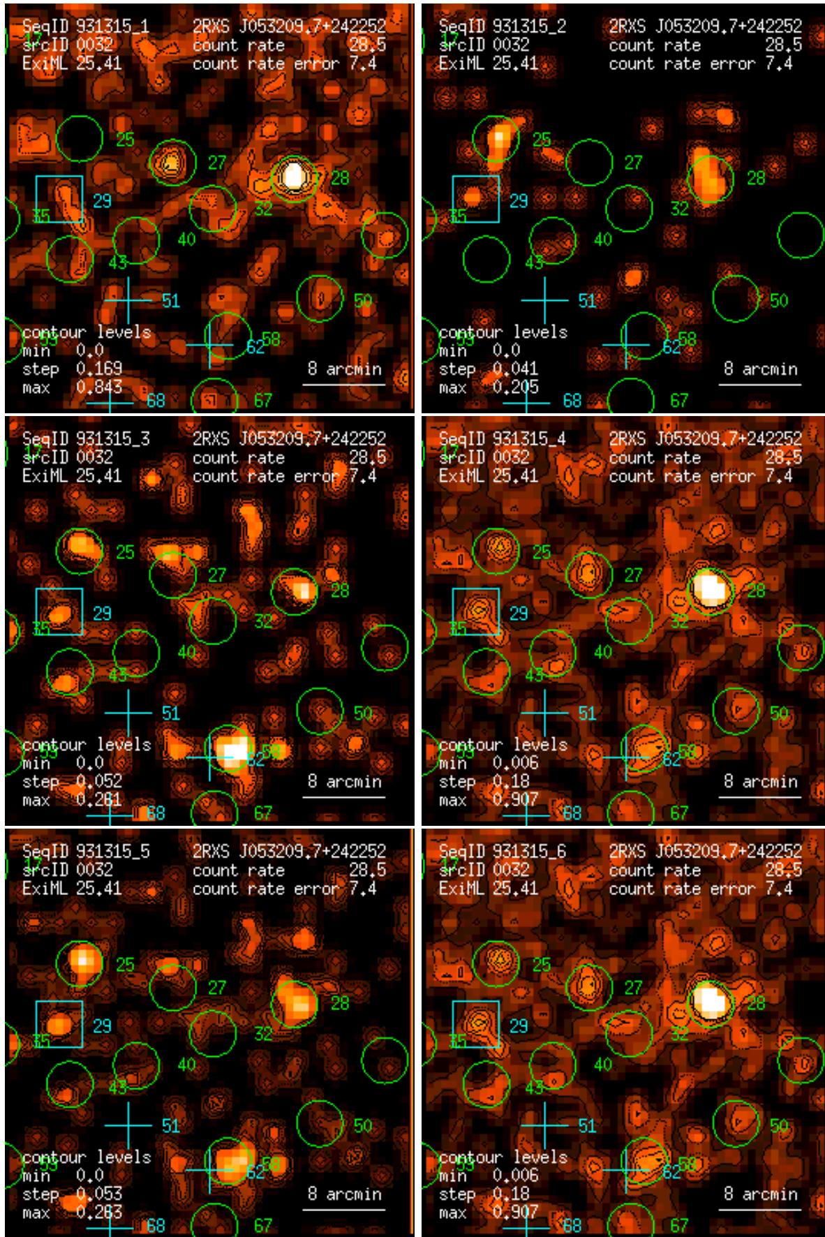
Figure 32: RASS 931315: detection 0032: band rate images, Gaussian filter: (1) PSPC channels 11 – 41, (2) 52 – 90, (3) 91 – 201, (4) 11 – 235, (5) 52 – 201, (6) 11 – 201. Broad band rates in counts/ks. Band rate contour levels in counts/ks/arcmin 2 .
