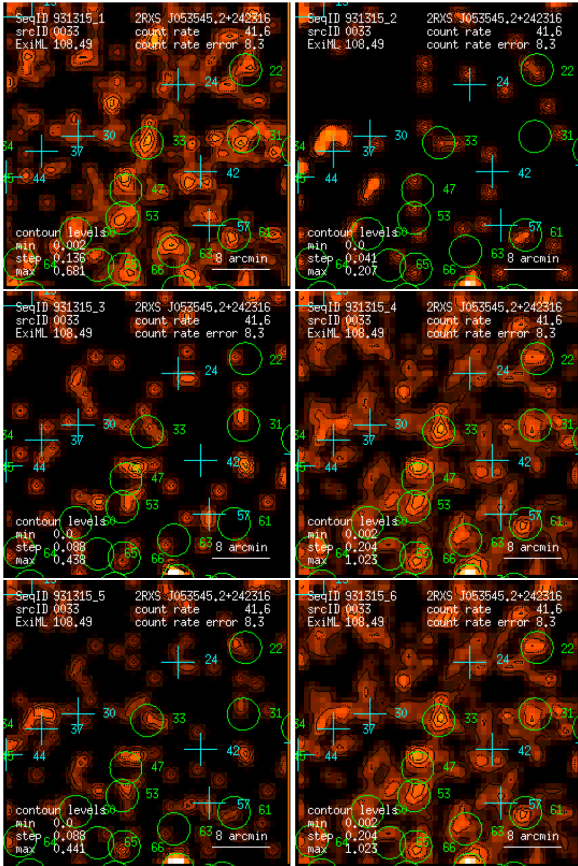
Figure 33: RASS 931315: detection 0033: band rate images, Gaussian filter: (1) PSPC channels 11 – 41, (2) 52 – 90, (3) 91 – 201, (4) 11 – 235, (5) 52 – 201, (6) 11 – 201. Broad band rates in counts/ks. Band rate contour levels in counts/ks/arcmin 2 .
