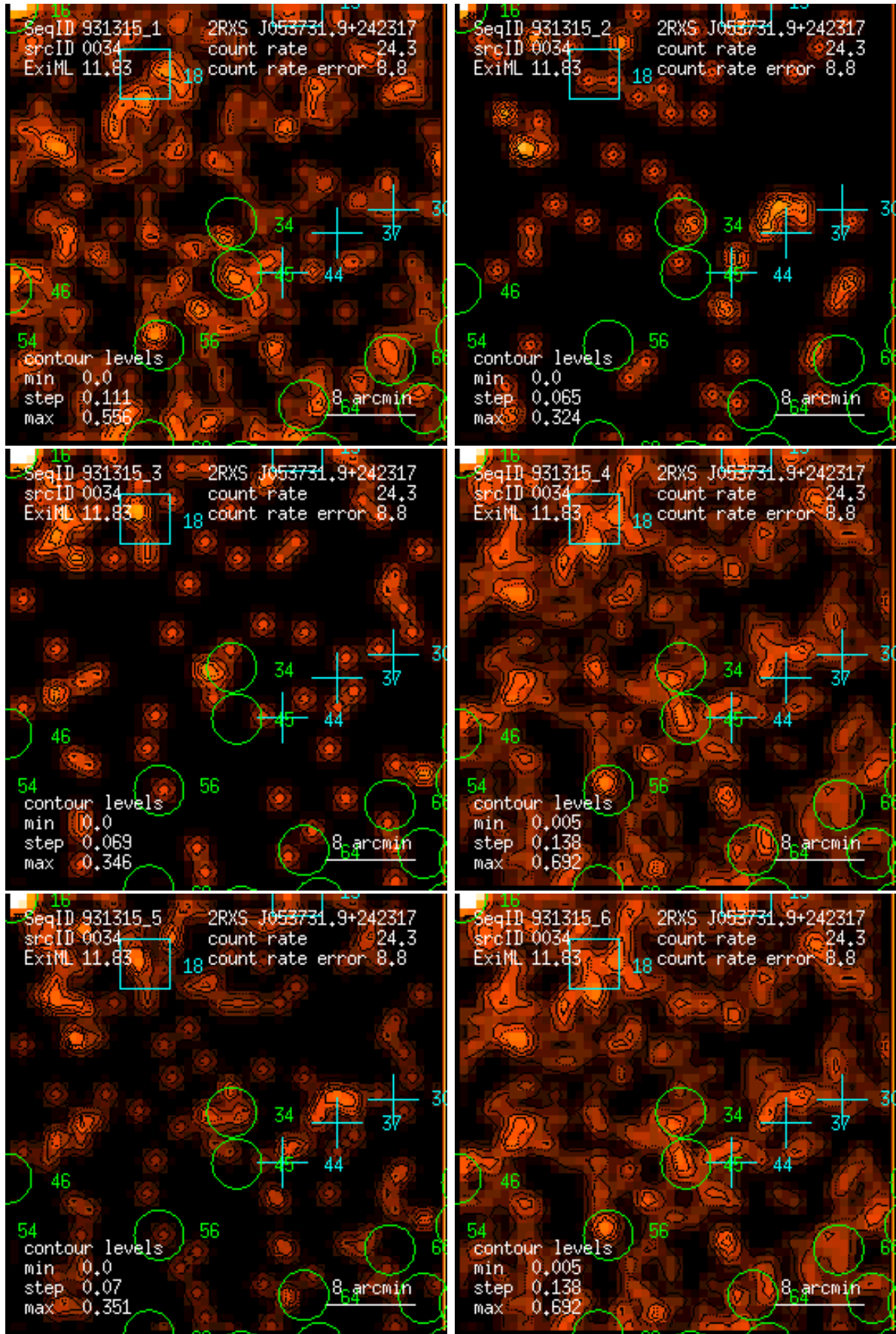
Figure 34: RASS 931315: detection 0034: band rate images, Gaussian filter: (1) PSPC channels 11 – 41, (2) 52 – 90, (3) 91 – 201, (4) 11 – 235, (5) 52 – 201, (6) 11 – 201. Broad band rates in counts/ks. Band rate contour levels in counts/ks/arcmin 2 .
