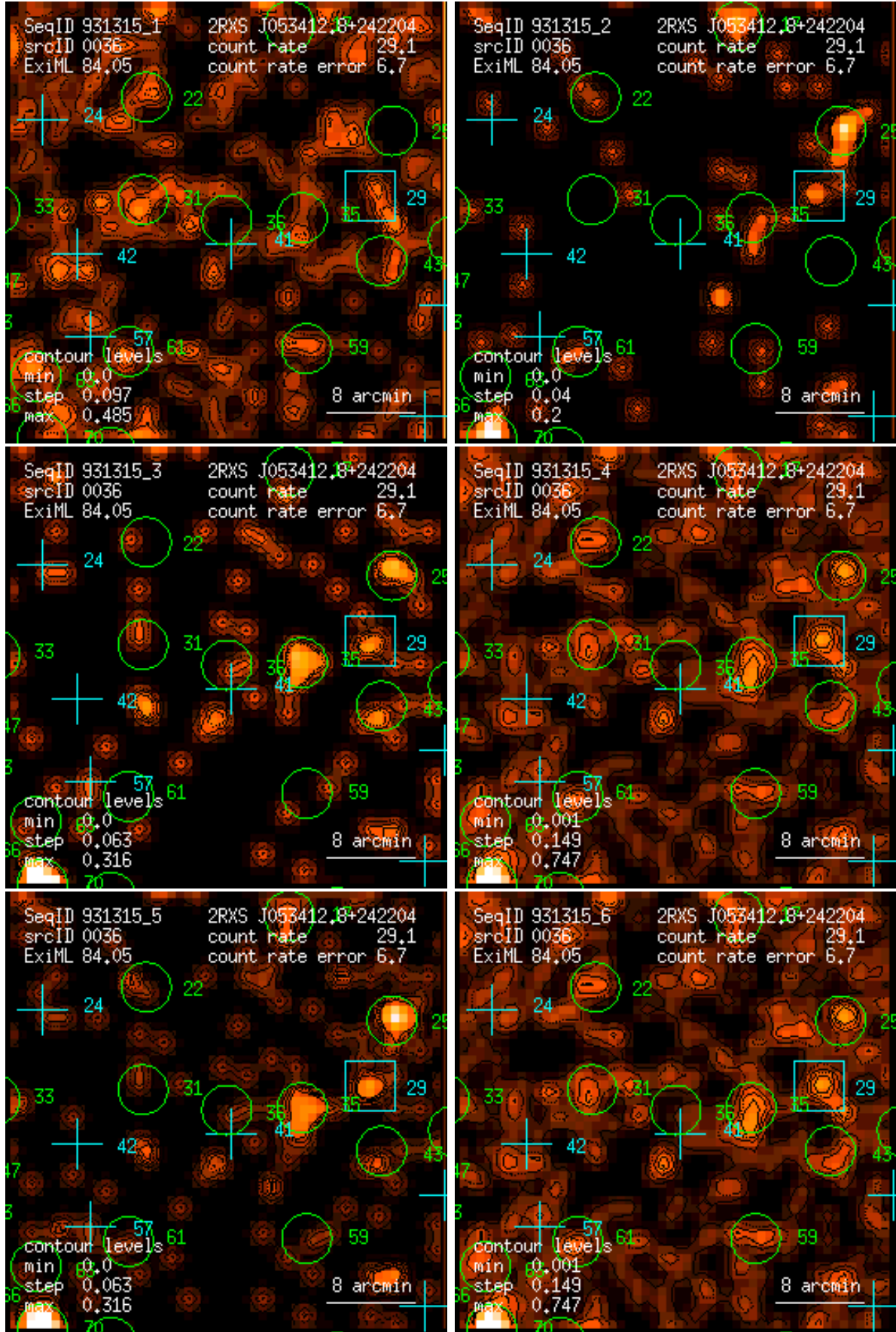
Figure 36: RASS 931315: detection 0036: band rate images, Gaussian filter: (1) PSPC channels 11 – 41, (2) 52 – 90, (3) 91 – 201, (4) 11 – 235, (5) 52 – 201, (6) 11 – 201. Broad band rates in counts/ks. Band rate contour levels in counts/ks/arcmin 2 .
