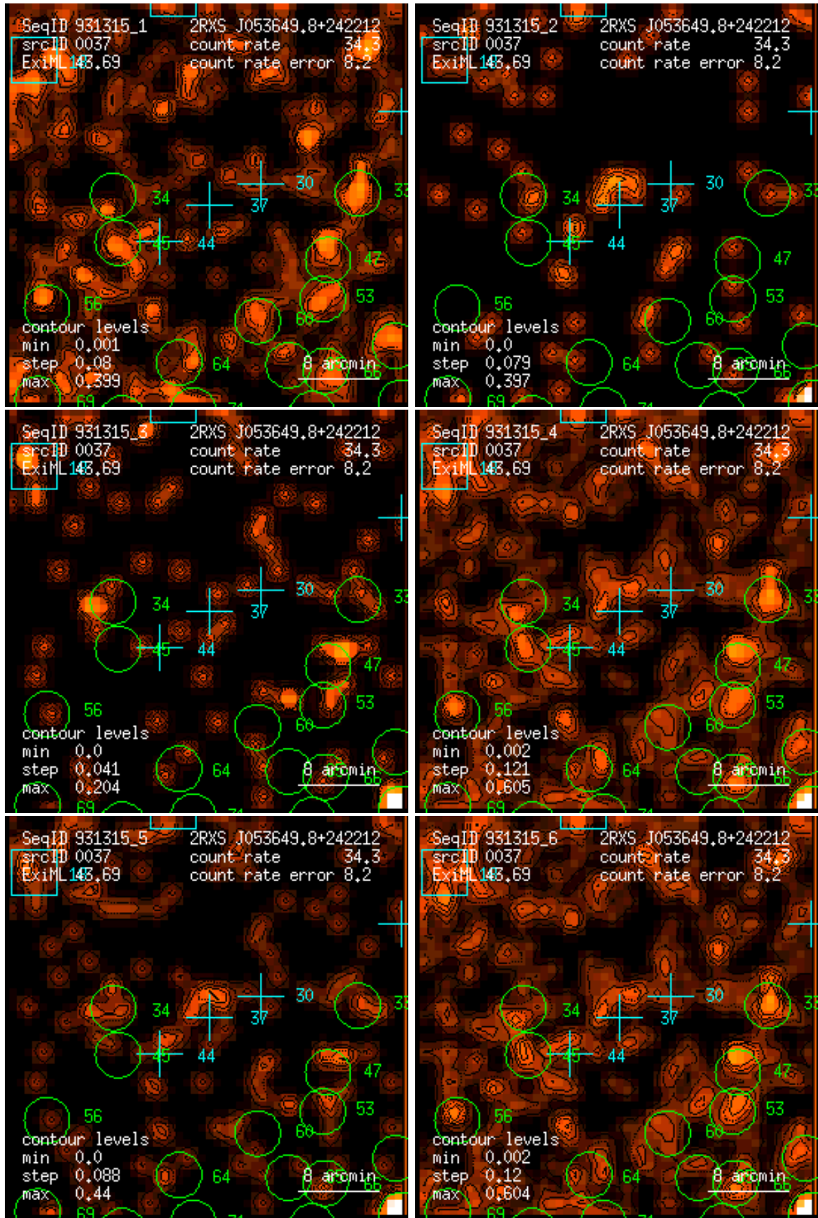
Figure 37: RASS 931315: detection 0037: band rate images, Gaussian filter: (1) PSPC channels 11 – 41, (2) 52 – 90, (3) 91 – 201, (4) 11 – 235, (5) 52 – 201, (6) 11 – 201. Broad band rates in counts/ks. Band rate contour levels in counts/ks/arcmin 2 .
