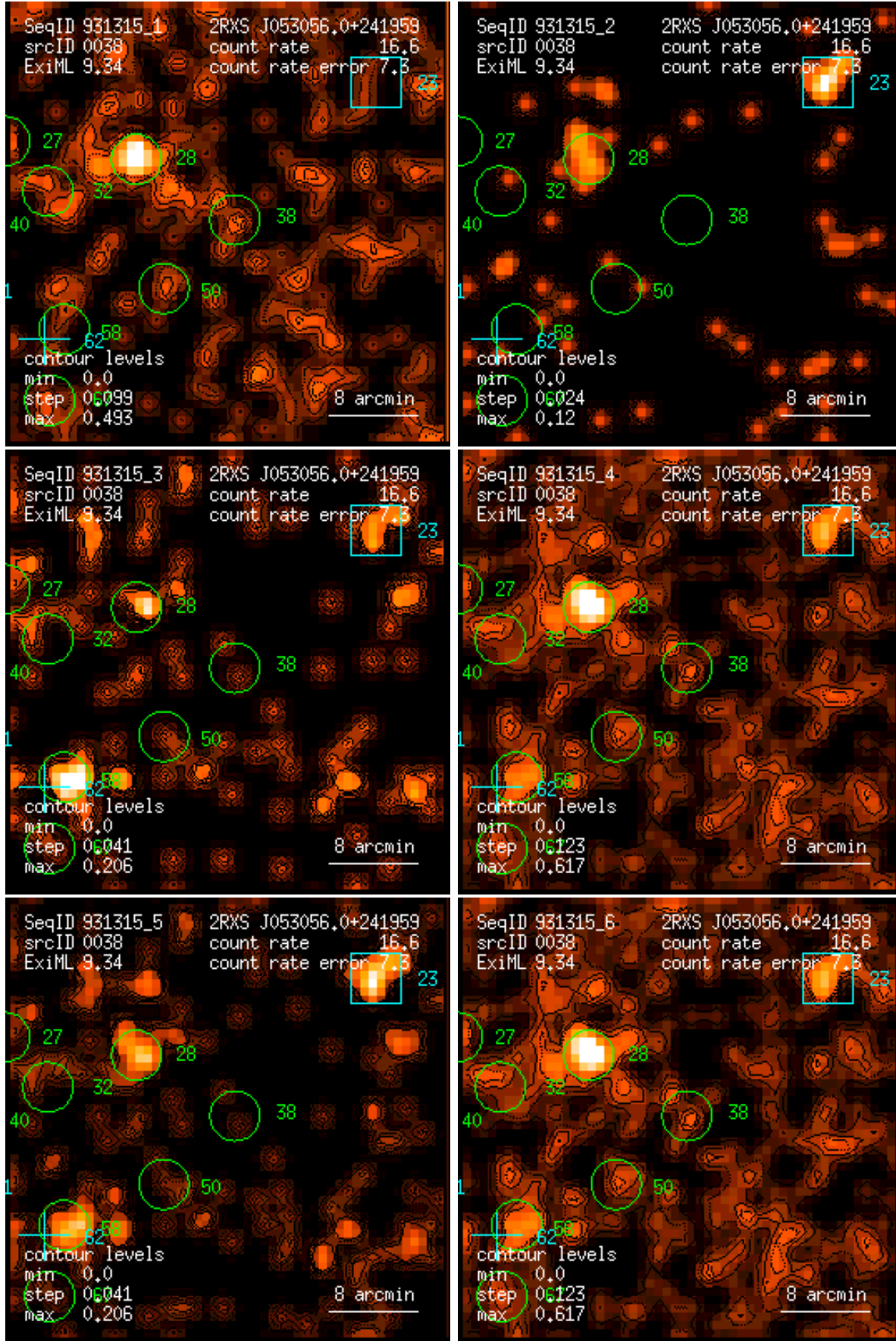
Figure 38: RASS 931315: detection 0038: band rate images, Gaussian filter: (1) PSPC channels 11 – 41, (2) 52 – 90, (3) 91 – 201, (4) 11 – 235, (5) 52 – 201, (6) 11 – 201. Broad band rates in counts/ks. Band rate contour levels in counts/ks/arcmin 2 .
