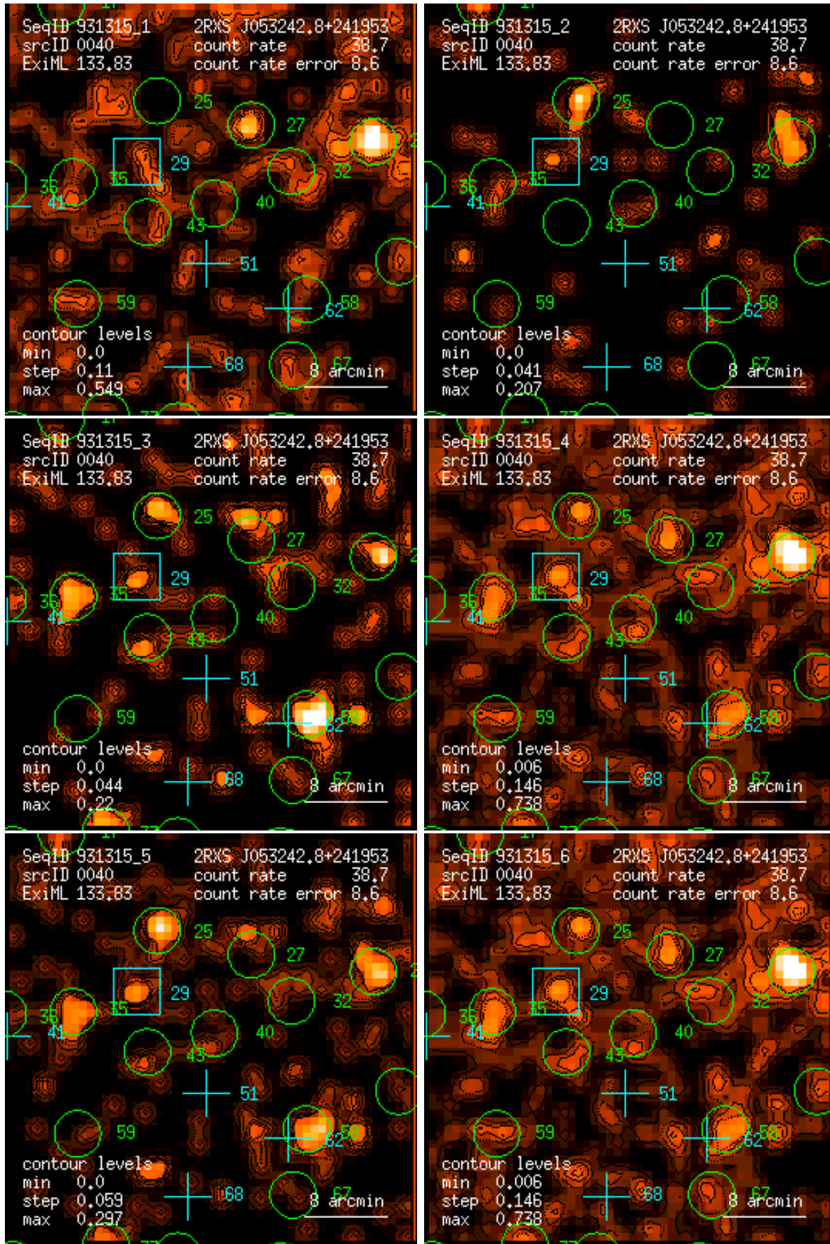
Figure 40: RASS 931315: detection 0040: band rate images, Gaussian filter: (1) PSPC channels 11 – 41, (2) 52 – 90, (3) 91 – 201, (4) 11 – 235, (5) 52 – 201, (6) 11 – 201. Broad band rates in counts/ks. Band rate contour levels in counts/ks/arcmin 2 .
