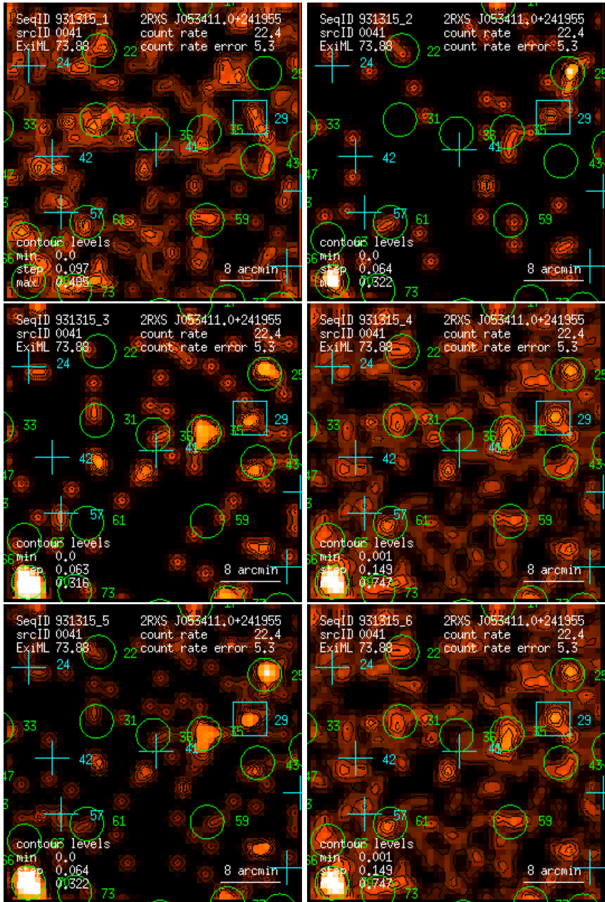
Figure 41: RASS 931315: detection 0041: band rate images, Gaussian filter: (1) PSPC channels 11 – 41, (2) 52 – 90, (3) 91 – 201, (4) 11 – 235, (5) 52 – 201, (6) 11 – 201. Broad band rates in counts/ks. Band rate contour levels in counts/ks/arcmin 2 .
