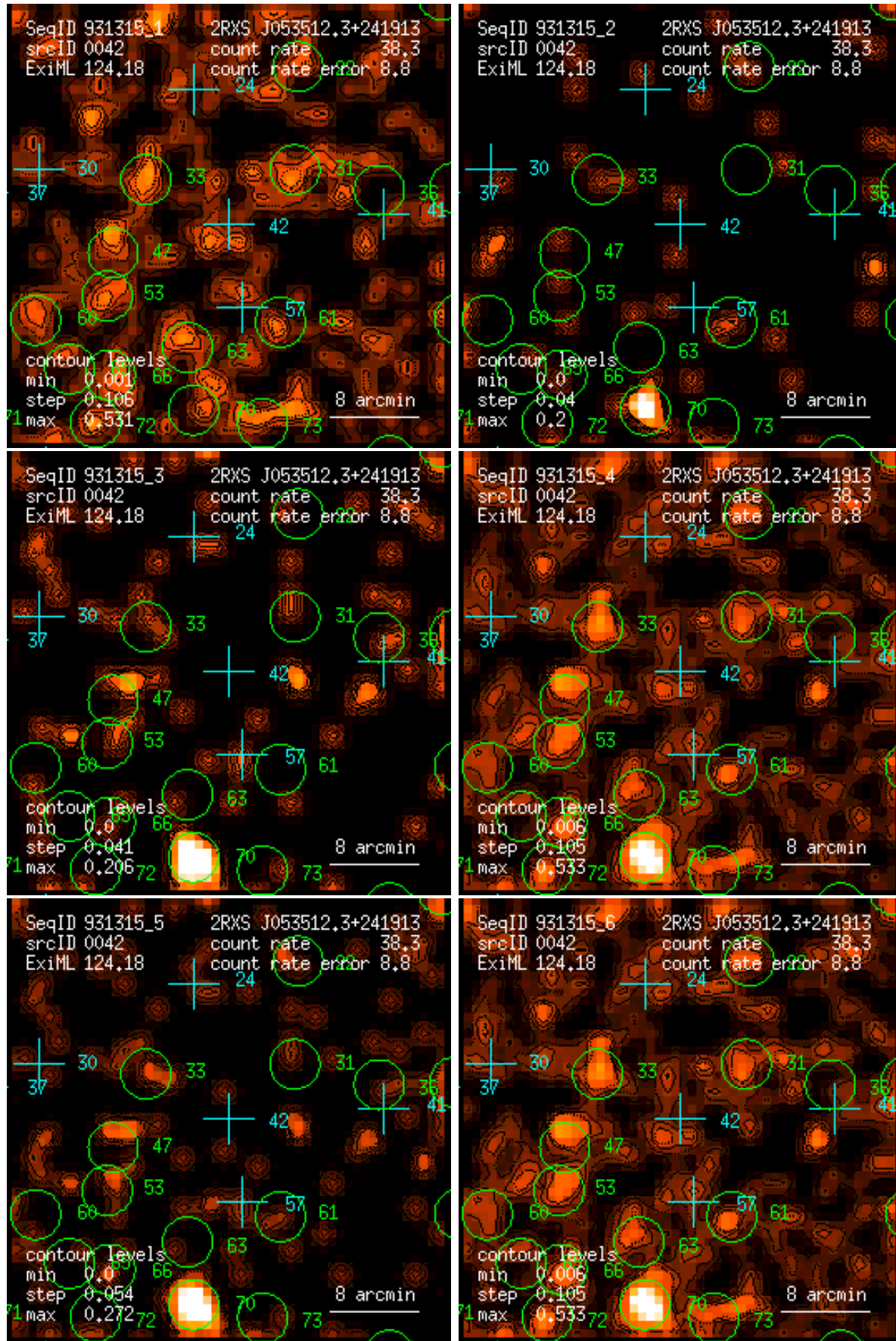
Figure 42: RASS 931315: detection 0042: band rate images, Gaussian filter: (1) PSPC channels 11 – 41, (2) 52 – 90, (3) 91 – 201, (4) 11 – 235, (5) 52 – 201, (6) 11 – 201. Broad band rates in counts/ks. Band rate contour levels in counts/ks/arcmin 2 .
