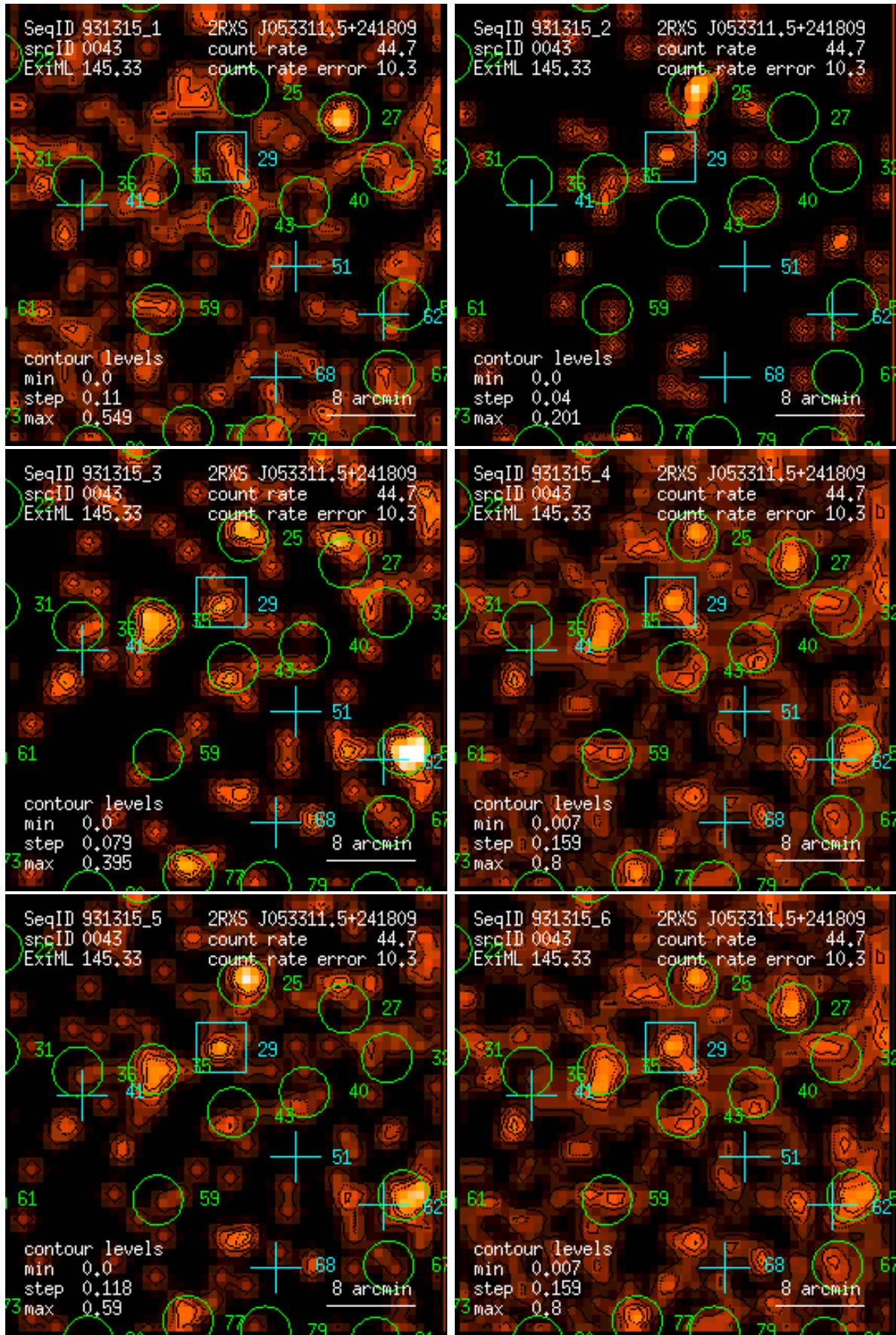
Figure 43: RASS 931315: detection 0043: band rate images, Gaussian filter: (1) PSPC channels 11 – 41, (2) 52 – 90, (3) 91 – 201, (4) 11 – 235, (5) 52 – 201, (6) 11 – 201. Broad band rates in counts/ks. Band rate contour levels in counts/ks/arcmin 2 .
