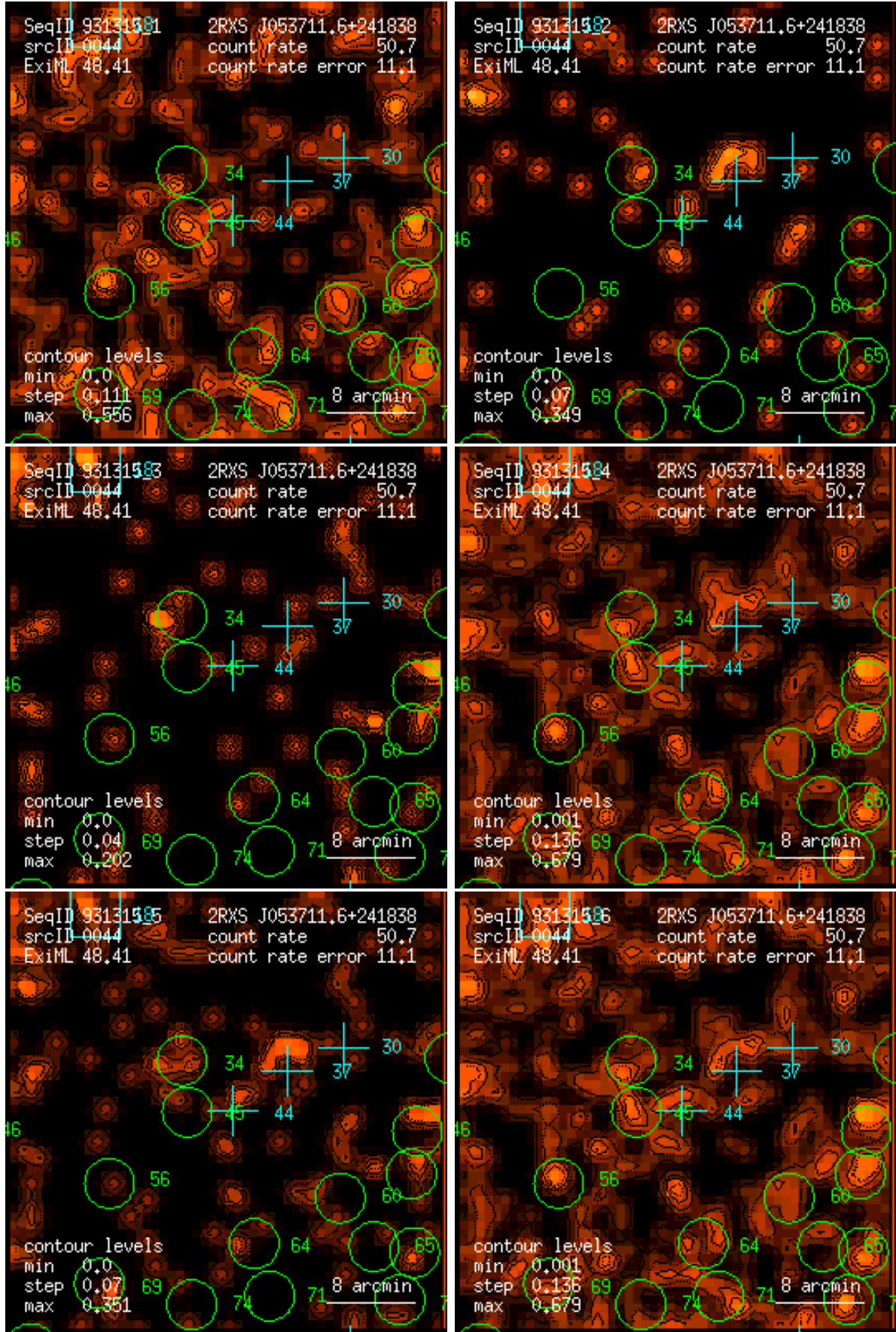
Figure 44: RASS 931315: detection 0044: band rate images, Gaussian filter: (1) PSPC channels 11 – 41, (2) 52 – 90, (3) 91 – 201, (4) 11 – 235, (5) 52 – 201, (6) 11 – 201. Broad band rates in counts/ks. Band rate contour levels in counts/ks/arcmin 2 .
