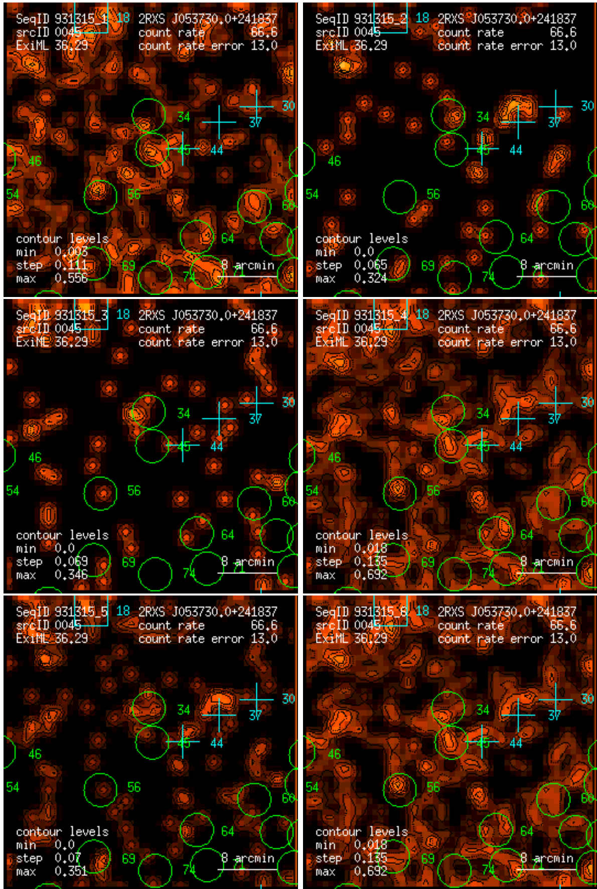
Figure 45: RASS 931315: detection 0045: band rate images, Gaussian filter: (1) PSPC channels 11 – 41, (2) 52 – 90, (3) 91 – 201, (4) 11 – 235, (5) 52 – 201, (6) 11 – 201. Broad band rates in counts/ks. Band rate contour levels in counts/ks/arcmin 2 .
