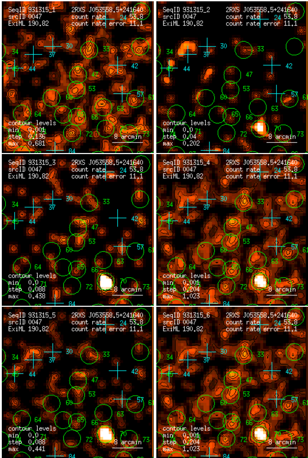
Figure 47: RASS 931315: detection 0047: band rate images, Gaussian filter: (1) PSPC channels 11 – 41, (2) 52 – 90, (3) 91 – 201, (4) 11 – 235, (5) 52 – 201, (6) 11 – 201. Broad band rates in counts/ks. Band rate contour levels in counts/ks/arcmin 2 .
