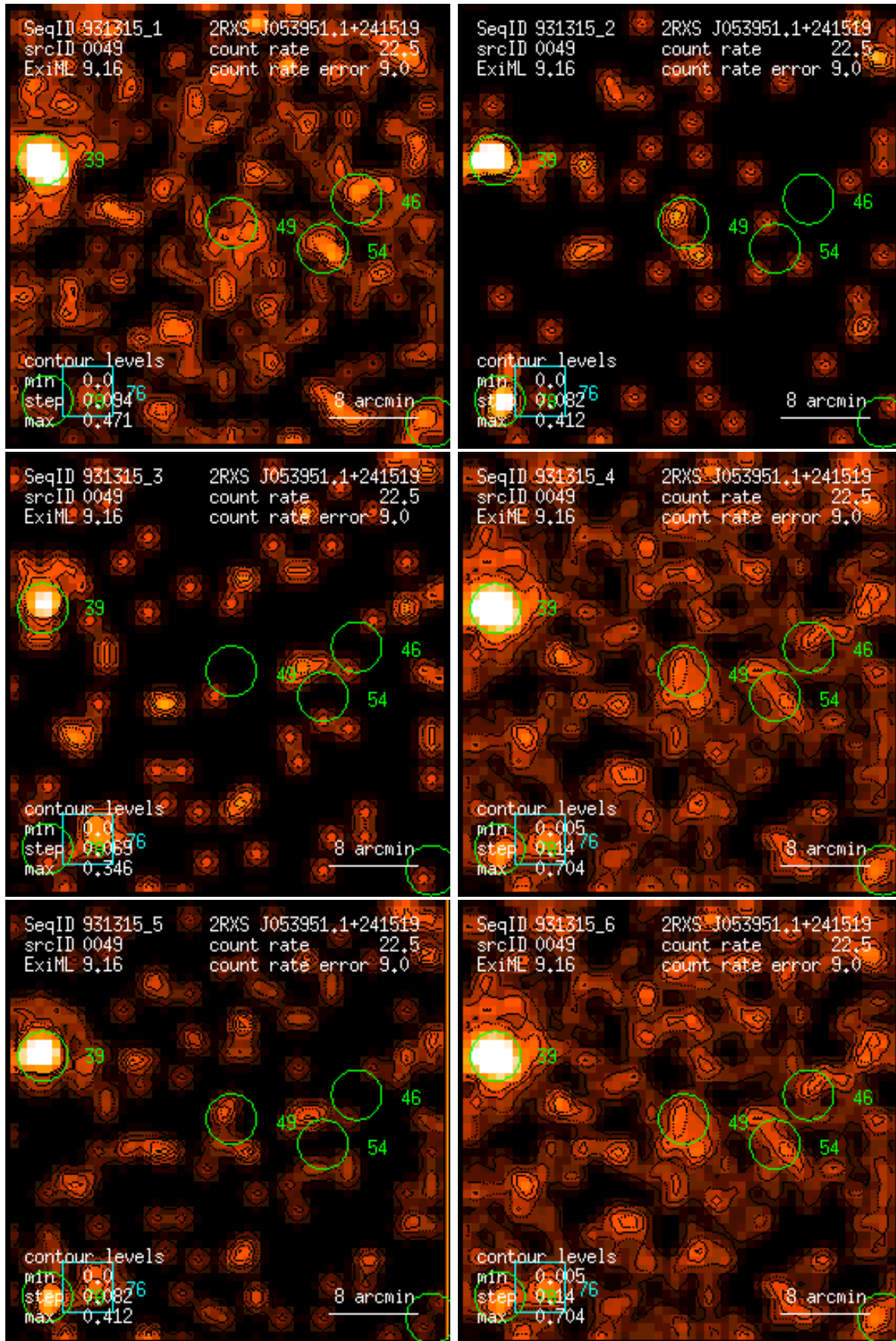
Figure 49: RASS 931315: detection 0049: band rate images, Gaussian filter: (1) PSPC channels 11 – 41, (2) 52 – 90, (3) 91 – 201, (4) 11 – 235, (5) 52 – 201, (6) 11 – 201. Broad band rates in counts/ks. Band rate contour levels in counts/ks/arcmin 2 .
