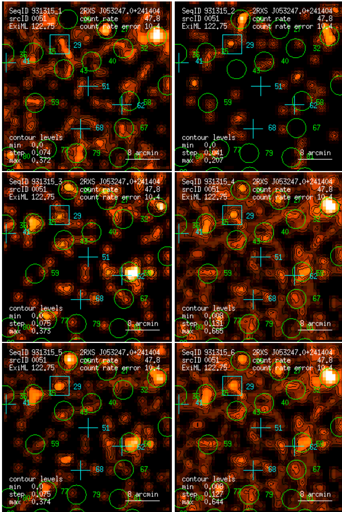
Figure 51: RASS 931315: detection 0051: band rate images, Gaussian filter: (1) PSPC channels 11 – 41, (2) 52 – 90, (3) 91 – 201, (4) 11 – 235, (5) 52 – 201, (6) 11 – 201. Broad band rates in counts/ks. Band rate contour levels in counts/ks/arcmin 2 .
