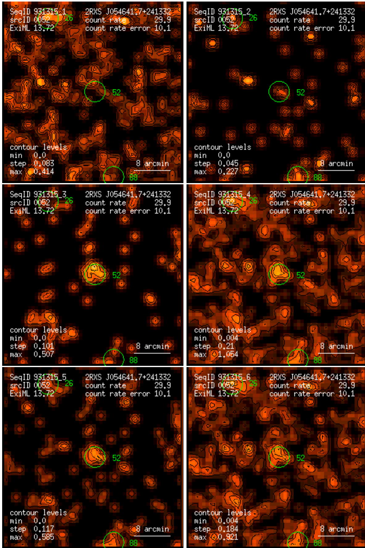
Figure 52: RASS 931315: detection 0052: band rate images, Gaussian filter: (1) PSPC channels 11 – 41, (2) 52 – 90, (3) 91 – 201, (4) 11 – 235, (5) 52 – 201, (6) 11 – 201. Broad band rates in counts/ks. Band rate contour levels in counts/ks/arcmin 2 .
