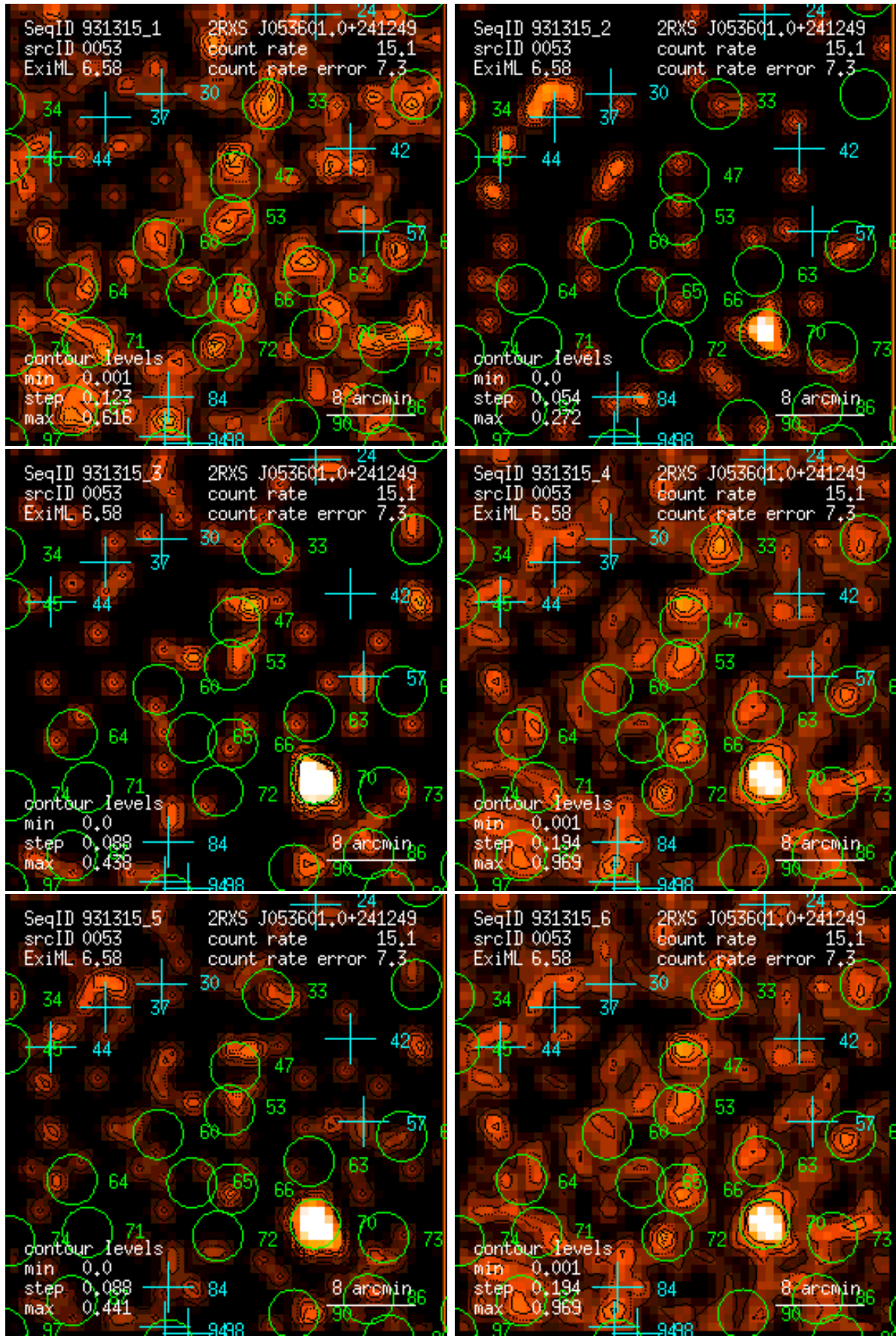
Figure 53: RASS 931315: detection 0053: band rate images, Gaussian filter: (1) PSPC channels 11 – 41, (2) 52 – 90, (3) 91 – 201, (4) 11 – 235, (5) 52 – 201, (6) 11 – 201. Broad band rates in counts/ks. Band rate contour levels in counts/ks/arcmin 2 .
