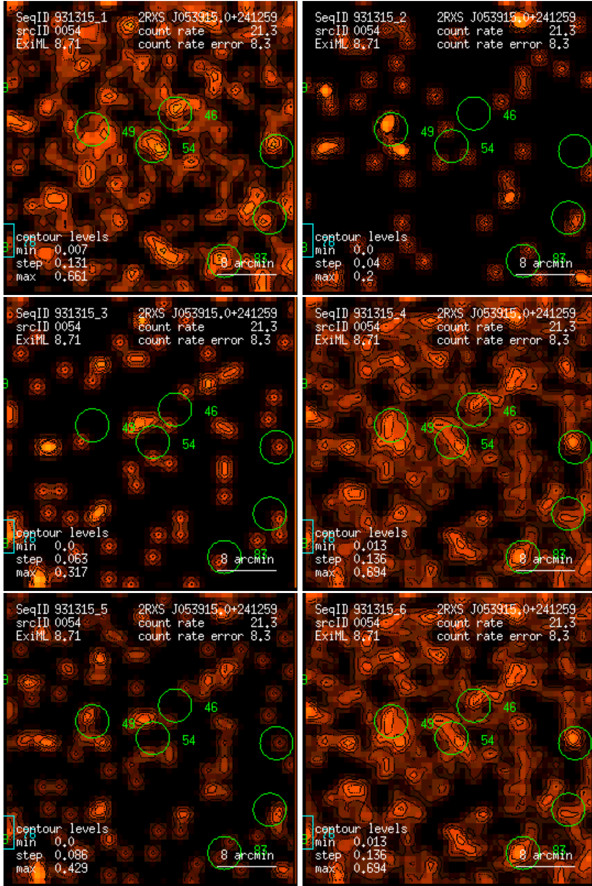
Figure 54: RASS 931315: detection 0054: band rate images, Gaussian filter: (1) PSPC channels 11 – 41, (2) 52 – 90, (3) 91 – 201, (4) 11 – 235, (5) 52 – 201, (6) 11 – 201. Broad band rates in counts/ks. Band rate contour levels in counts/ks/arcmin 2 .
