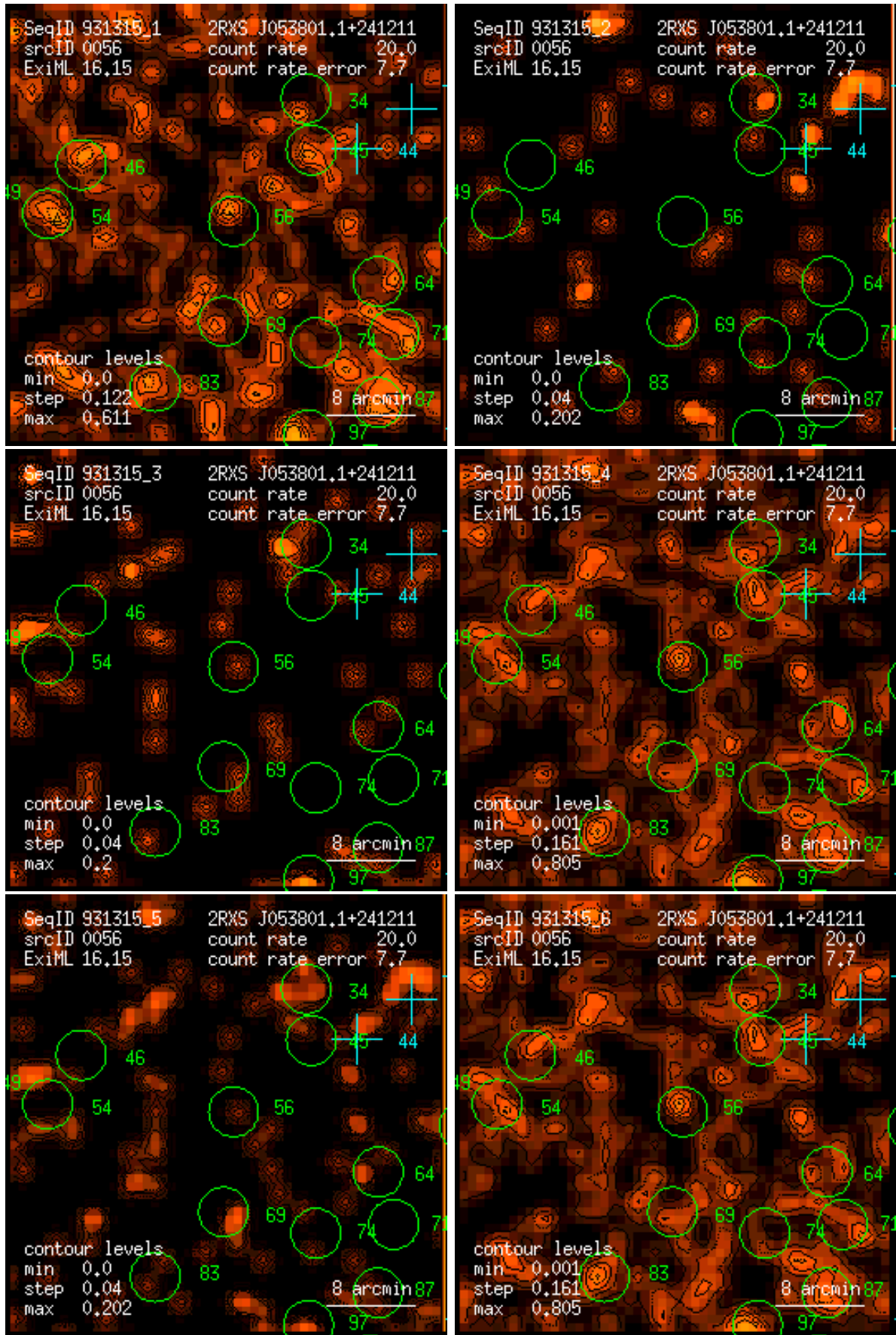
Figure 56: RASS 931315: detection 0056: band rate images, Gaussian filter: (1) PSPC channels 11 – 41, (2) 52 – 90, (3) 91 – 201, (4) 11 – 235, (5) 52 – 201, (6) 11 – 201. Broad band rates in counts/ks. Band rate contour levels in counts/ks/arcmin 2 .
