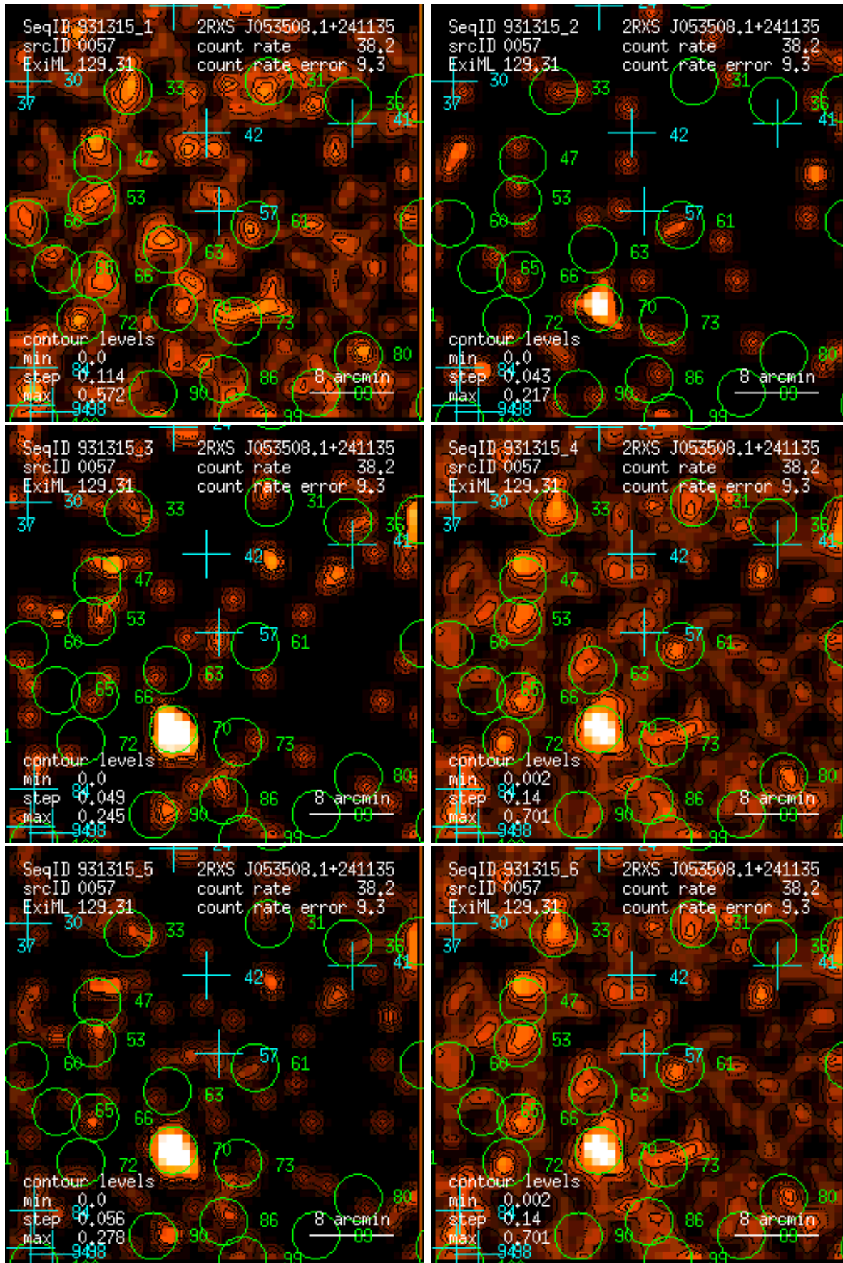
Figure 57: RASS 931315: detection 0057: band rate images, Gaussian filter: (1) PSPC channels 11 – 41, (2) 52 – 90, (3) 91 – 201, (4) 11 – 235, (5) 52 – 201, (6) 11 – 201. Broad band rates in counts/ks. Band rate contour levels in counts/ks/arcmin 2 .
