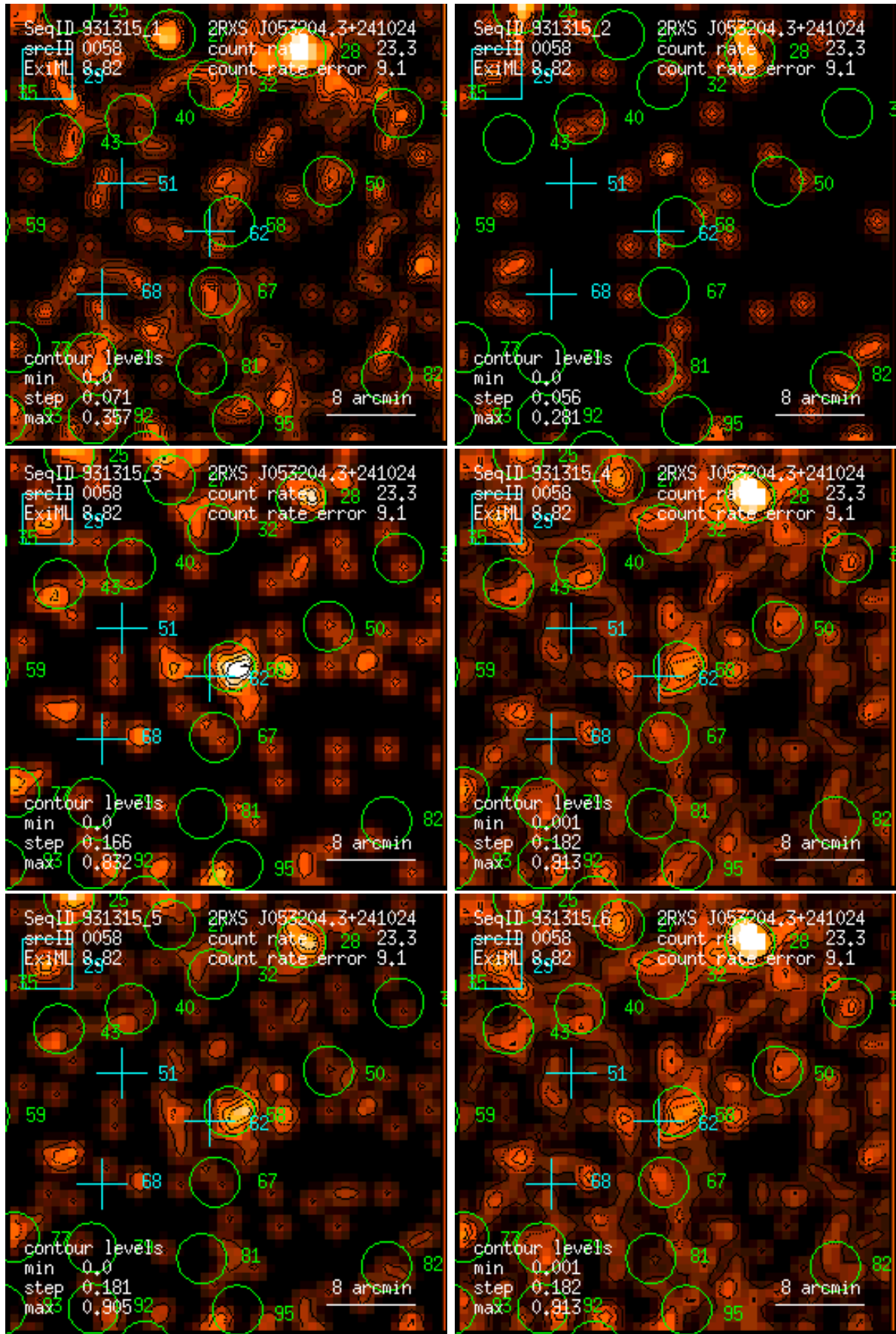
Figure 58: RASS 931315: detection 0058: band rate images, Gaussian filter: (1) PSPC channels 11 – 41, (2) 52 – 90, (3) 91 – 201, (4) 11 – 235, (5) 52 – 201, (6) 11 – 201. Broad band rates in counts/ks. Band rate contour levels in counts/ks/arcmin 2 .
