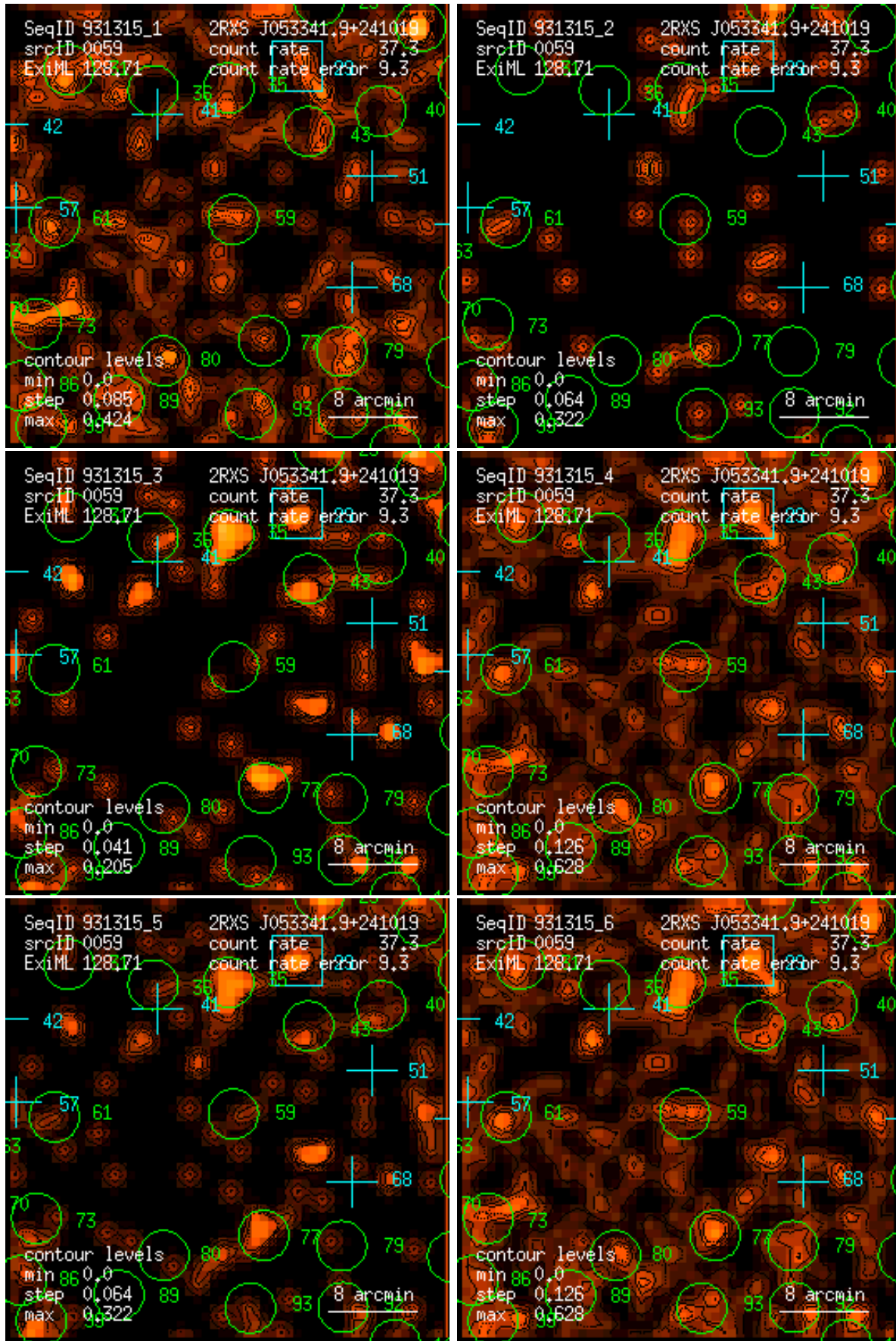
Figure 59: RASS 931315: detection 0059: band rate images, Gaussian filter: (1) PSPC channels 11 – 41, (2) 52 – 90, (3) 91 – 201, (4) 11 – 235, (5) 52 – 201, (6) 11 – 201. Broad band rates in counts/ks. Band rate contour levels in counts/ks/arcmin 2 .
