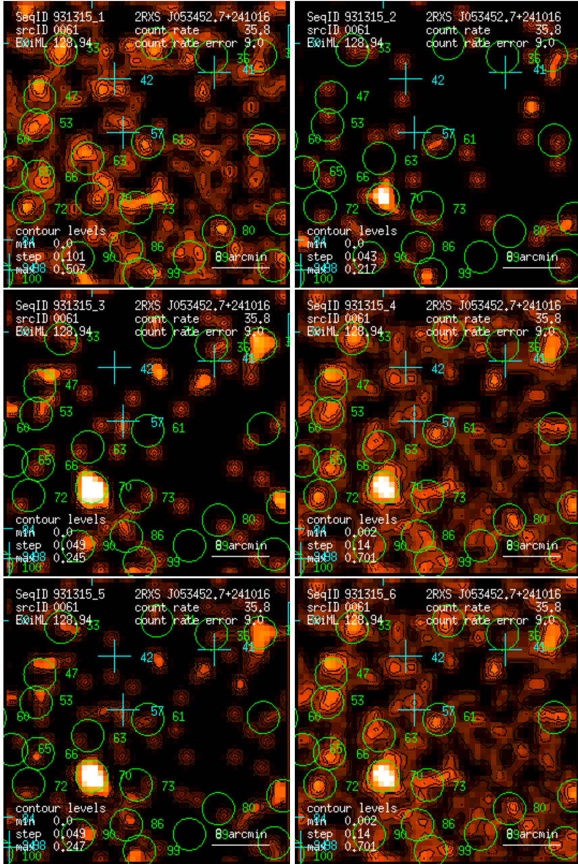
Figure 61: RASS 931315: detection 0061: band rate images, Gaussian filter: (1) PSPC channels 11 – 41, (2) 52 – 90, (3) 91 – 201, (4) 11 – 235, (5) 52 – 201, (6) 11 – 201. Broad band rates in counts/ks. Band rate contour levels in counts/ks/arcmin 2 .
