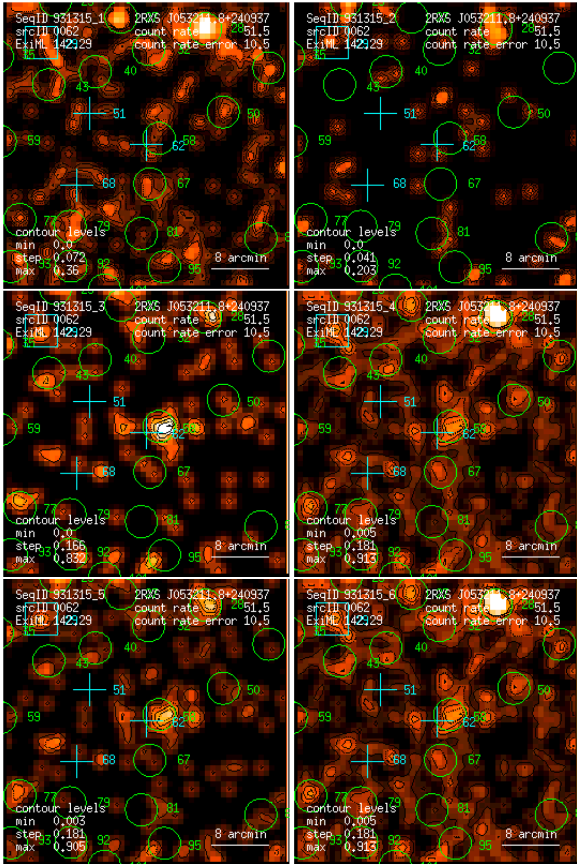
Figure 62: RASS 931315: detection 0062: band rate images, Gaussian filter: (1) PSPC channels 11 – 41, (2) 52 – 90, (3) 91 – 201, (4) 11 – 235, (5) 52 – 201, (6) 11 – 201. Broad band rates in counts/ks. Band rate contour levels in counts/ks/arcmin 2 .
