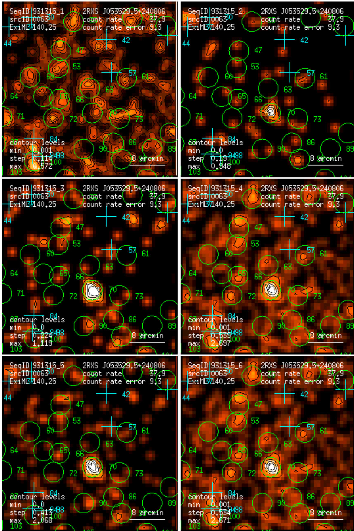
Figure 63: RASS 931315: detection 0063: band rate images, Gaussian filter: (1) PSPC channels 11 – 41, (2) 52 – 90, (3) 91 – 201, (4) 11 – 235, (5) 52 – 201, (6) 11 – 201. Broad band rates in counts/ks. Band rate contour levels in counts/ks/arcmin 2 .
