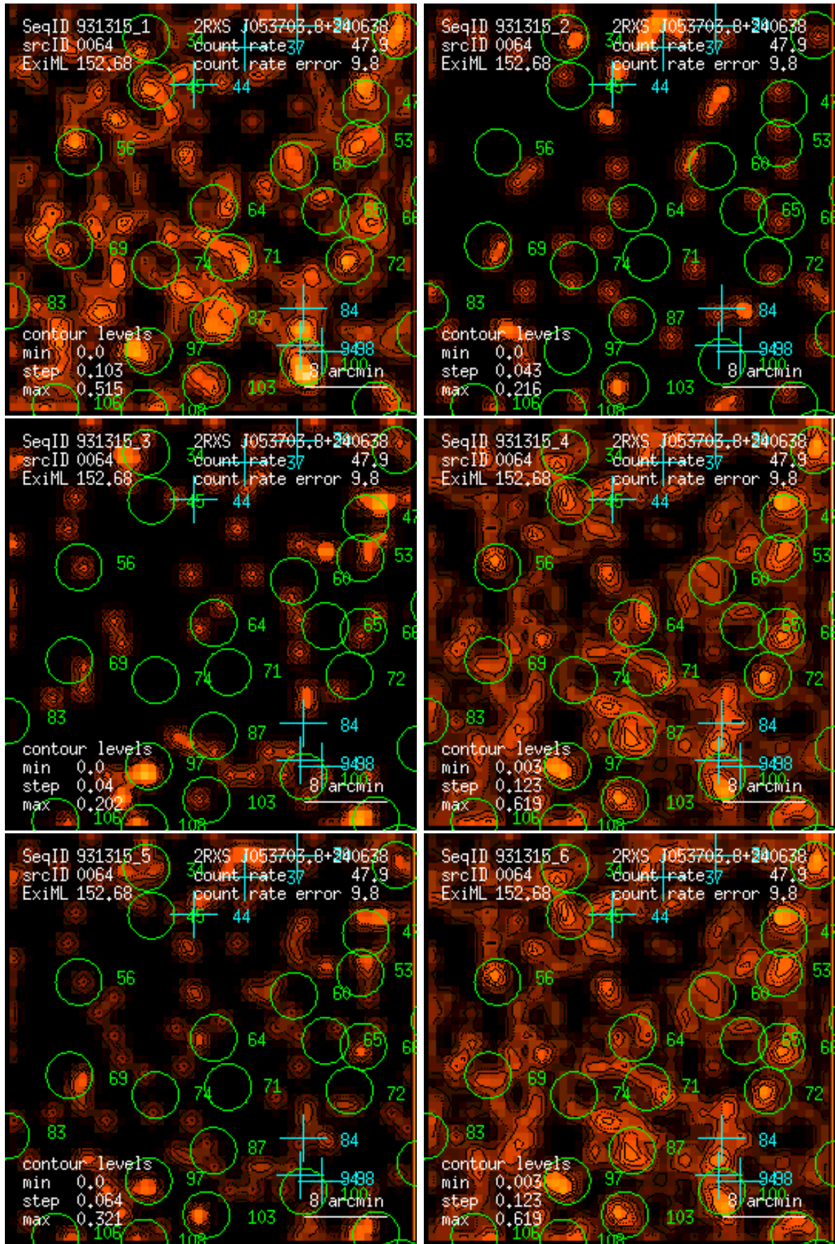
Figure 64: RASS 931315: detection 0064: band rate images, Gaussian filter: (1) PSPC channels 11 – 41, (2) 52 – 90, (3) 91 – 201, (4) 11 – 235, (5) 52 – 201, (6) 11 – 201. Broad band rates in counts/ks. Band rate contour levels in counts/ks/arcmin 2 .
