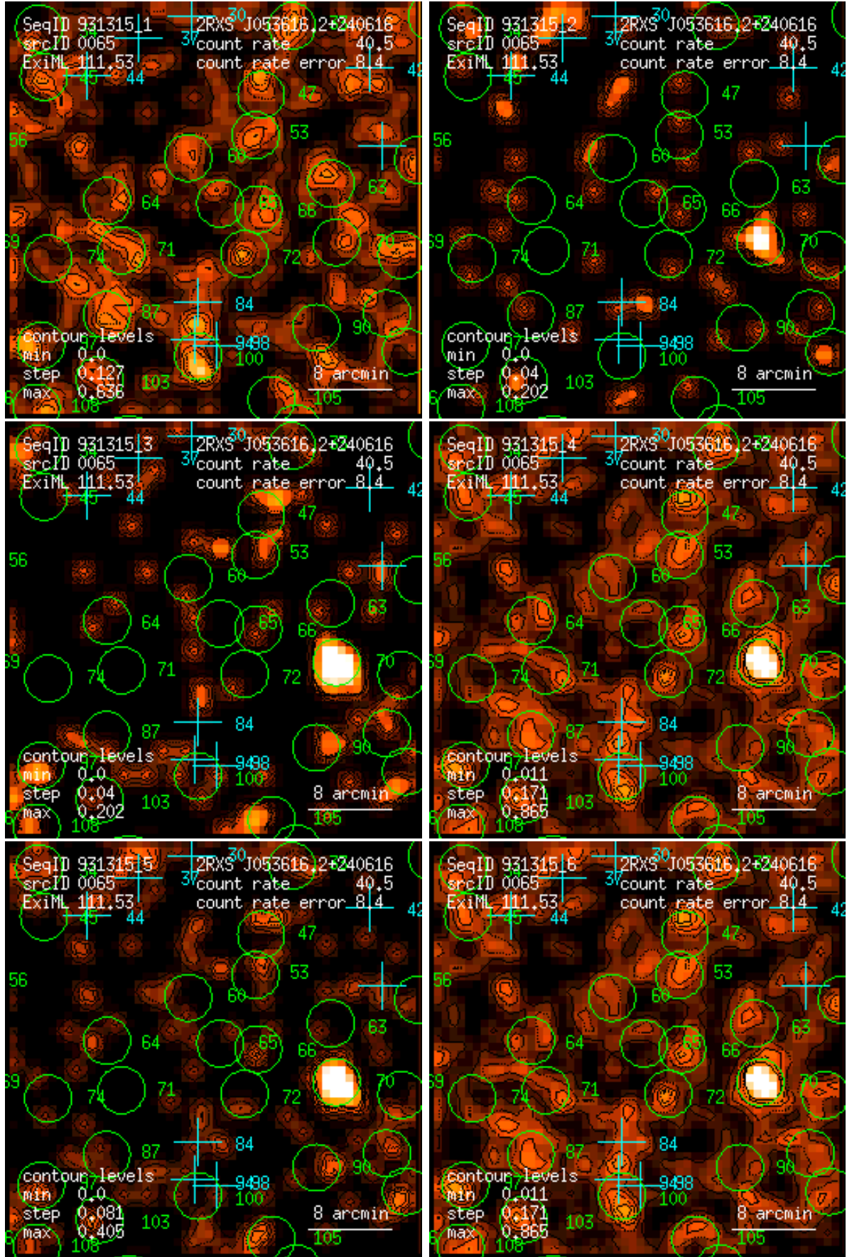
Figure 65: RASS 931315: detection 0065: band rate images, Gaussian filter: (1) PSPC channels 11 – 41, (2) 52 – 90, (3) 91 – 201, (4) 11 – 235, (5) 52 – 201, (6) 11 – 201. Broad band rates in counts/ks. Band rate contour levels in counts/ks/arcmin 2 .
