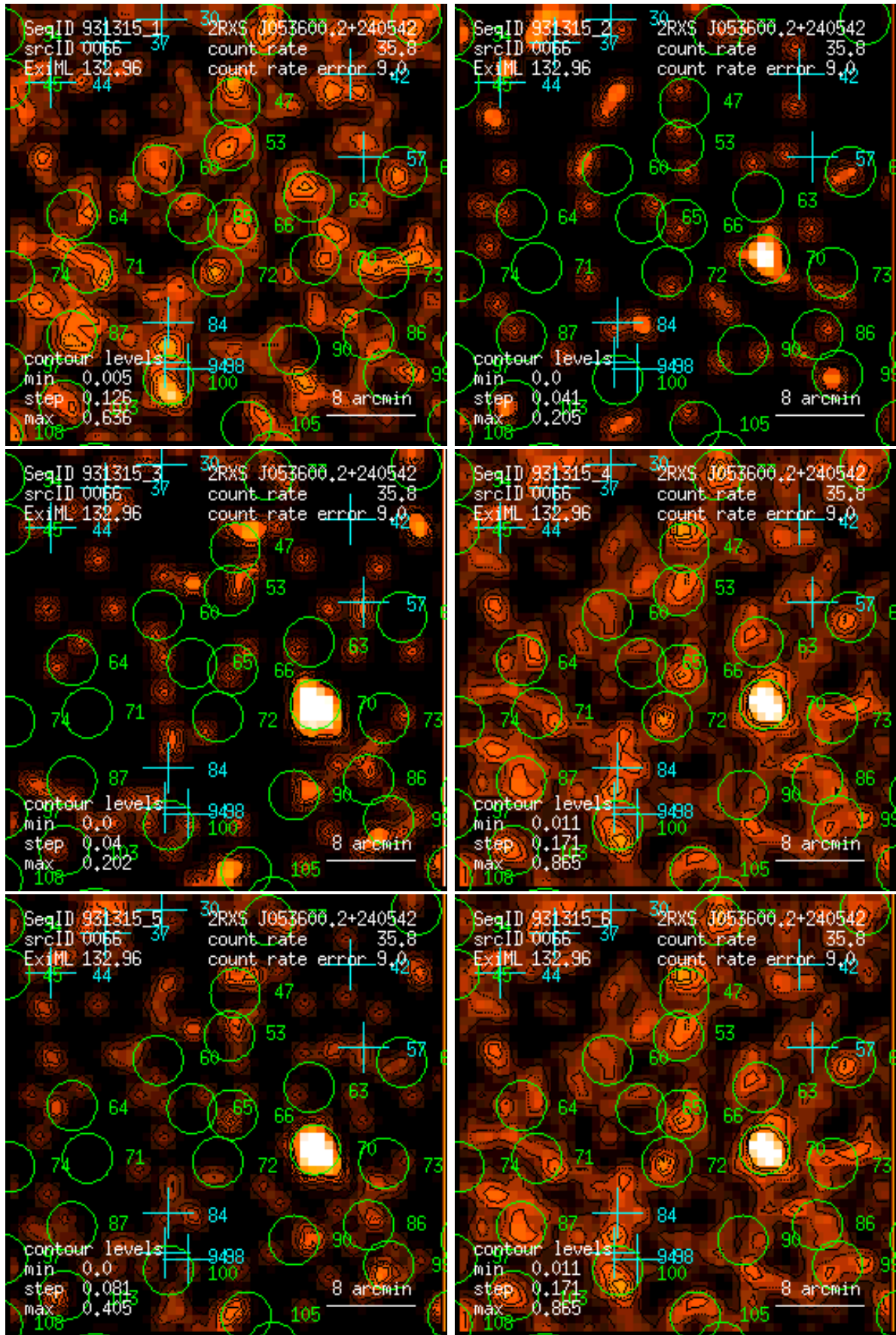
Figure 66: RASS 931315: detection 0066: band rate images, Gaussian filter: (1) PSPC channels 11 – 41, (2) 52 – 90, (3) 91 – 201, (4) 11 – 235, (5) 52 – 201, (6) 11 – 201. Broad band rates in counts/ks. Band rate contour levels in counts/ks/arcmin 2 .
