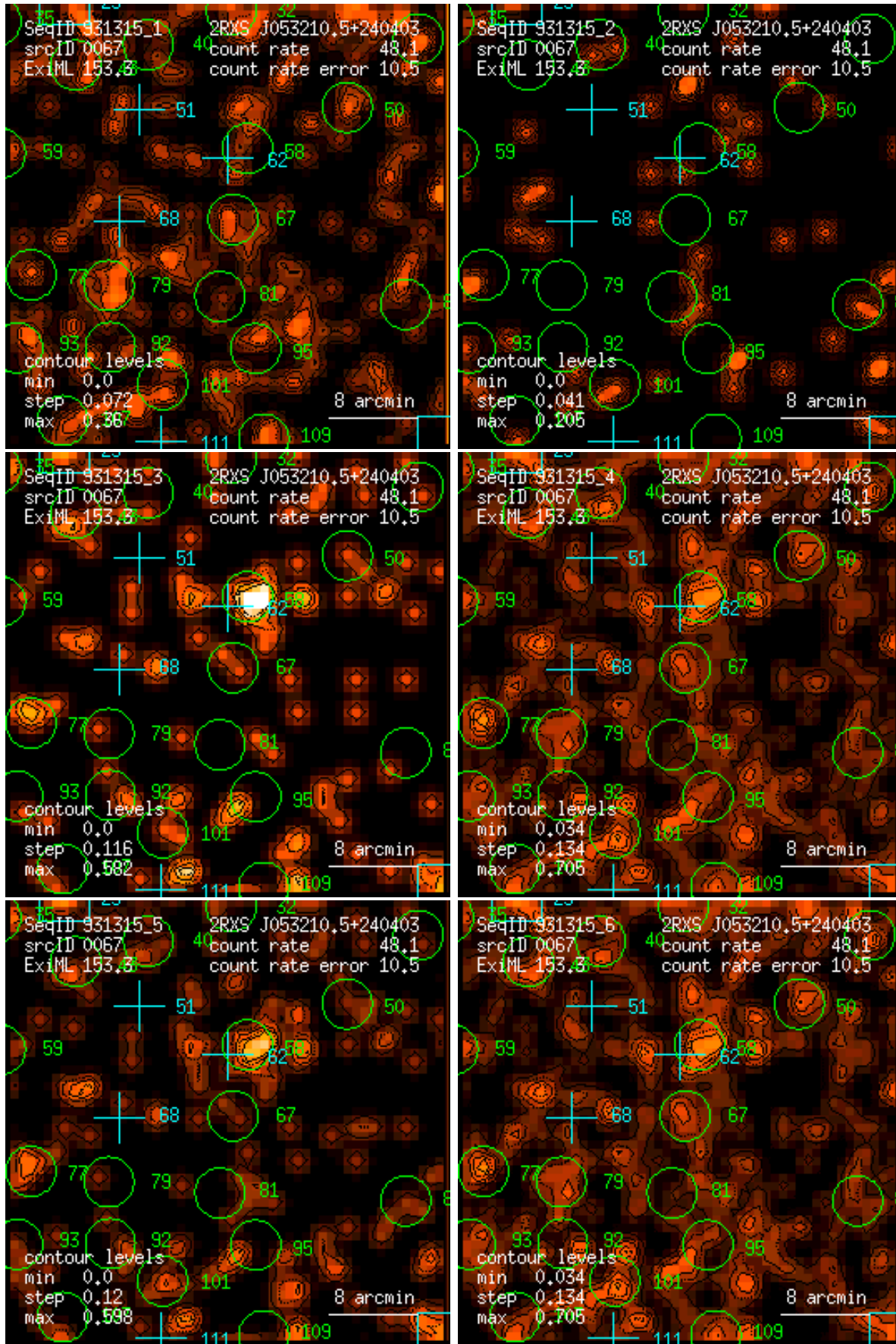
Figure 67: RASS 931315: detection 0067: band rate images, Gaussian filter: (1) PSPC channels 11 – 41, (2) 52 – 90, (3) 91 – 201, (4) 11 – 235, (5) 52 – 201, (6) 11 – 201. Broad band rates in counts/ks. Band rate contour levels in counts/ks/arcmin 2 .
